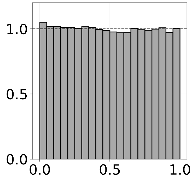
n = 100
