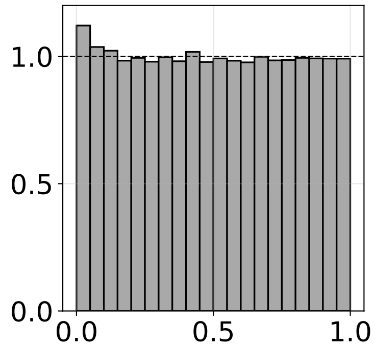
n = 1000
