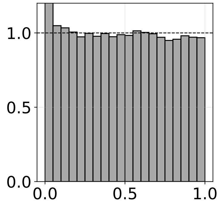
n = 500
