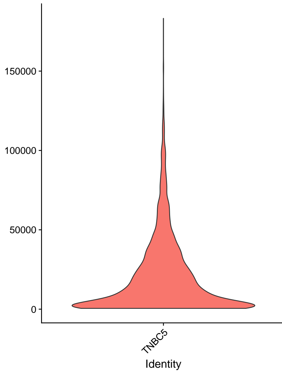
nCount_RNA
