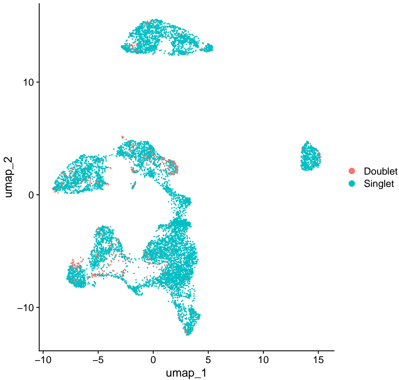
DF.classifications_0.25_0.005_588
