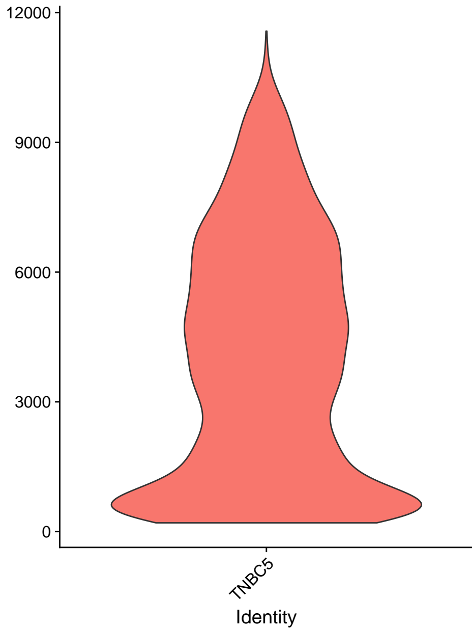
nFeature_RNA
