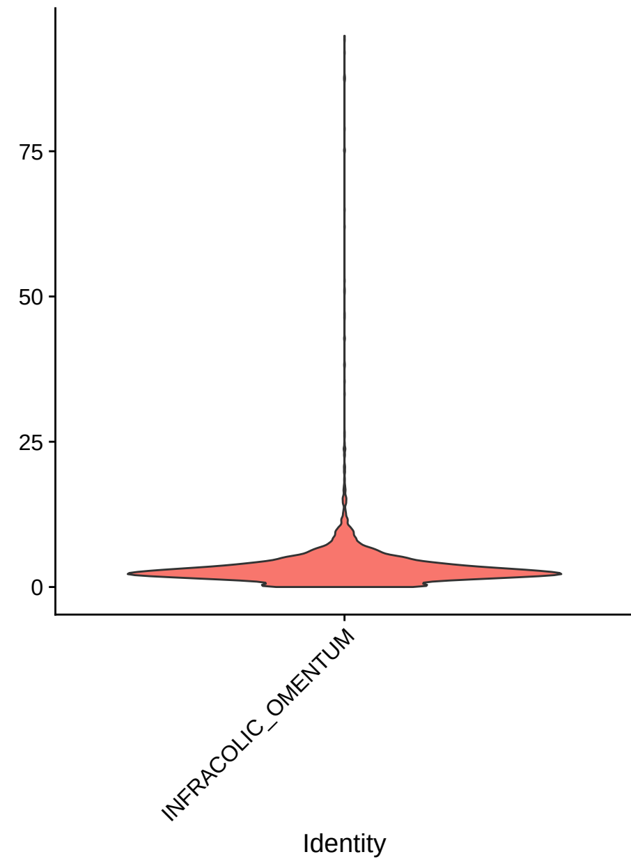
percent.mt
