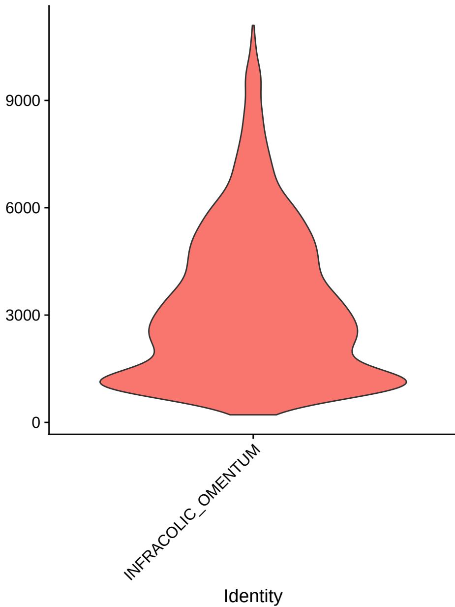
nFeature_RNA
