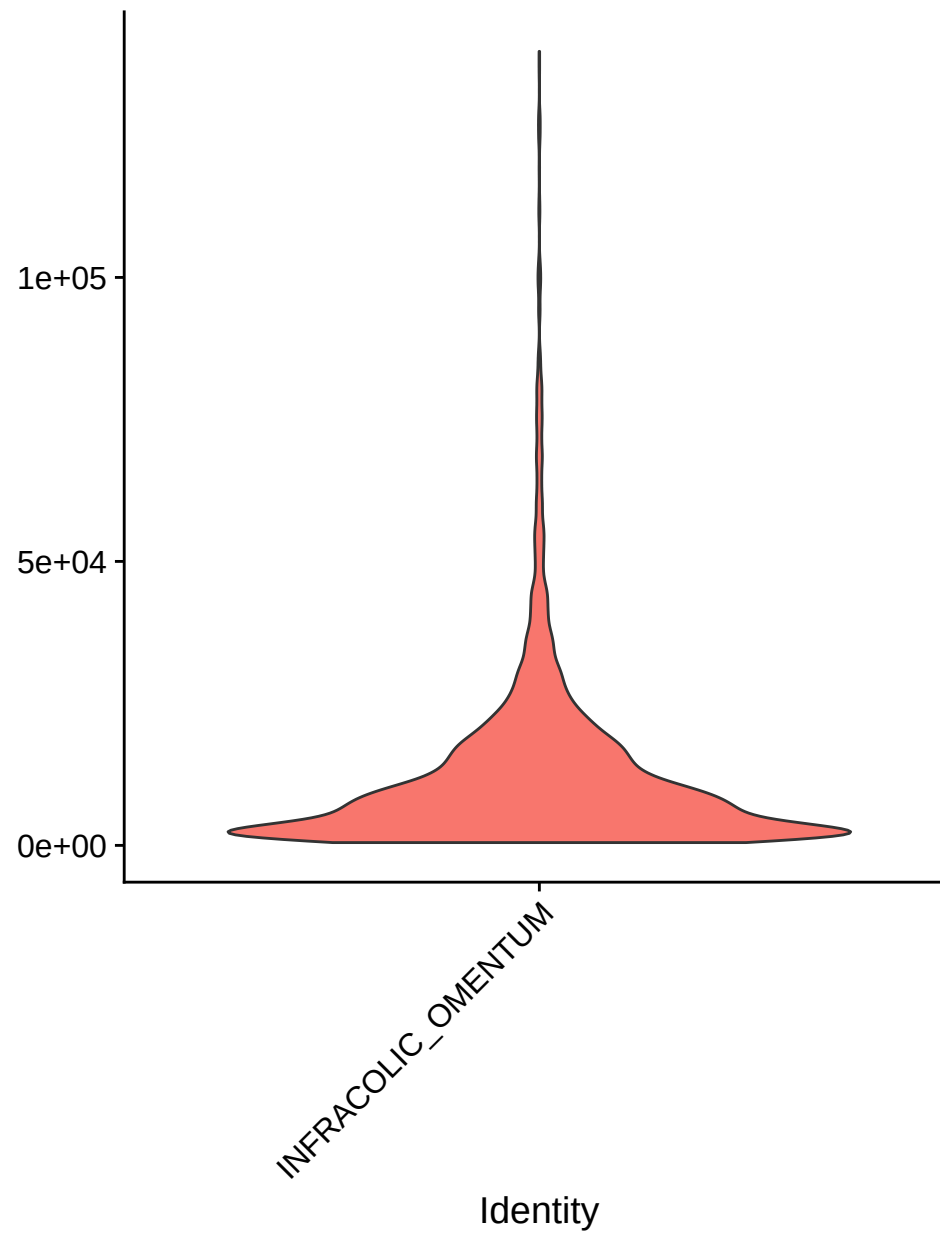
nCount_RNA
