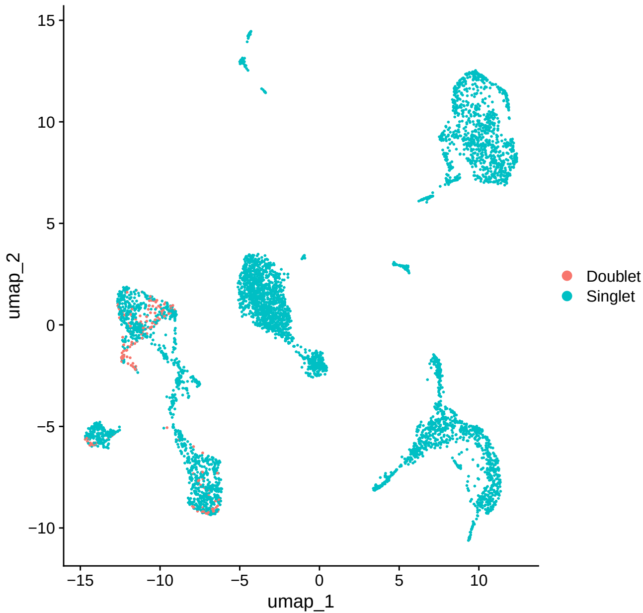
DF.classifications_0.25_0.19_171
