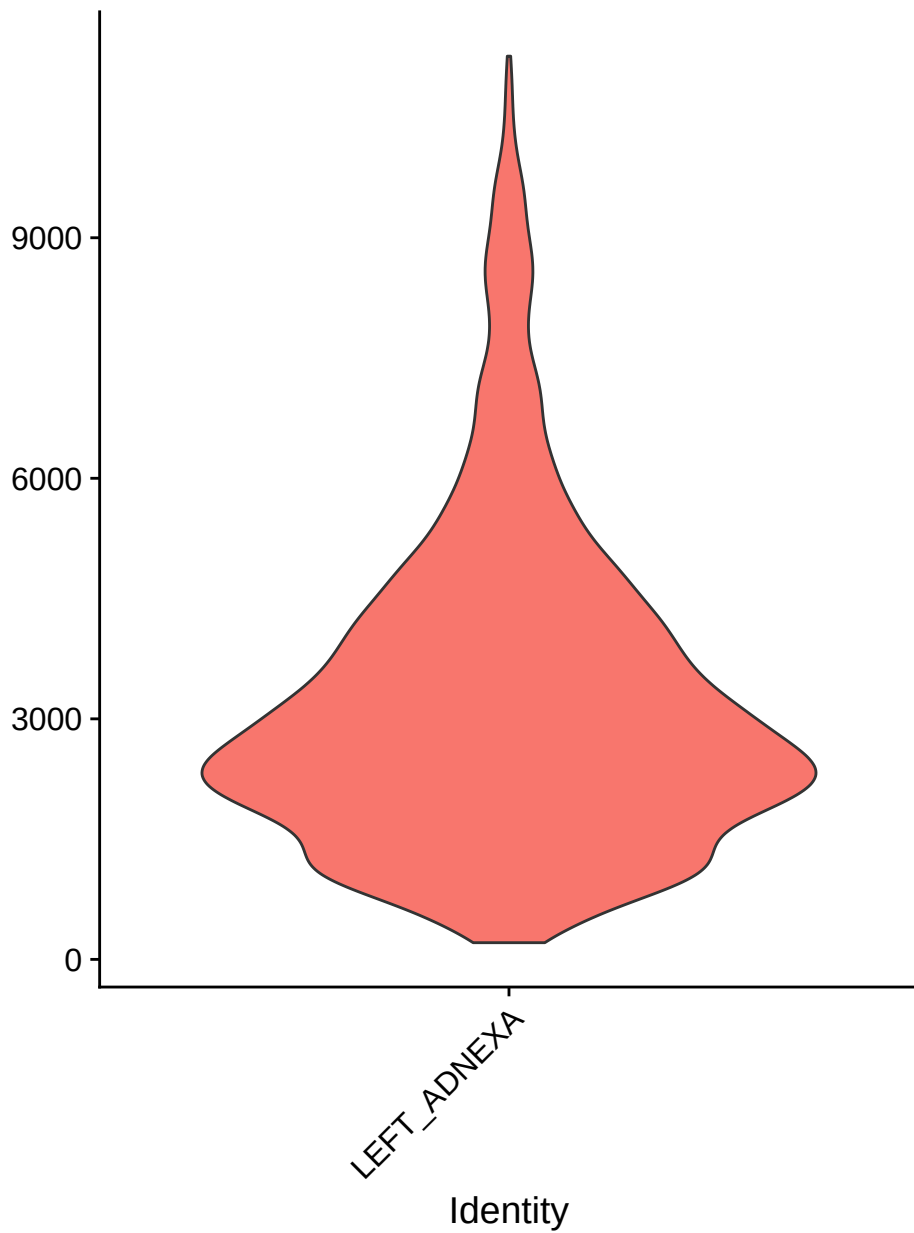
nFeature_RNA
