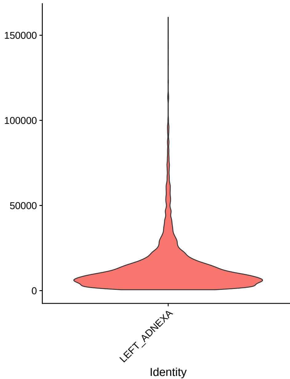
nCount_RNA
