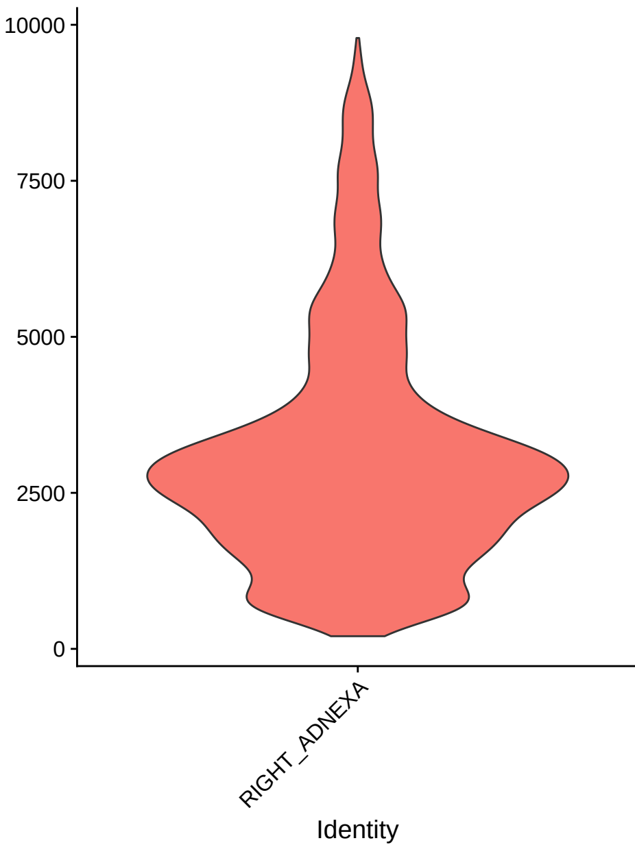
nFeature_RNA
