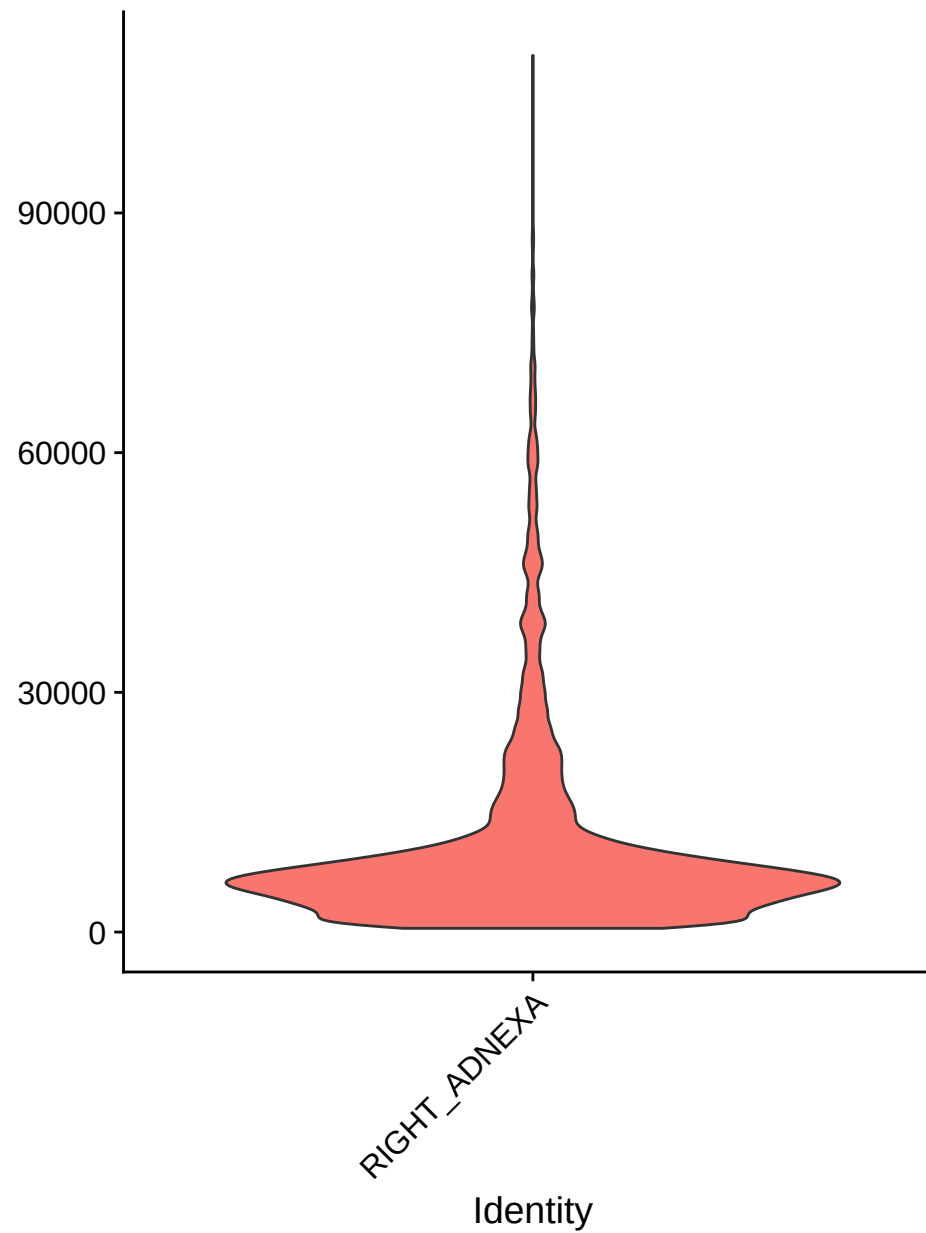
nCount_RNA
