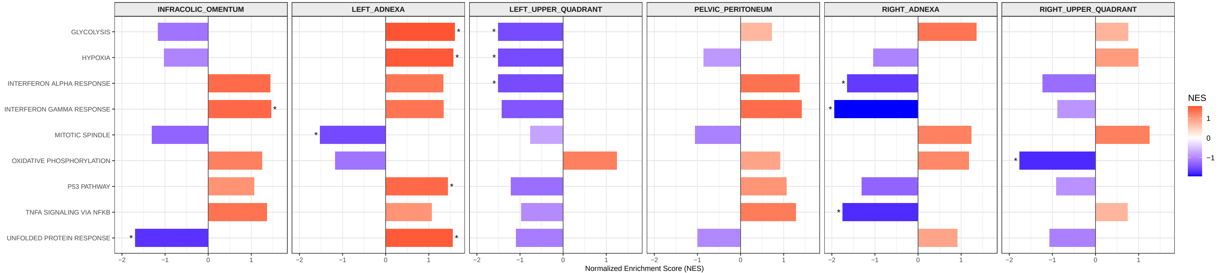
GSEA Hallmark – all_clones.by_sample.deg.tsv (padj < 0.05 | * = significant | no bar = not detected)
