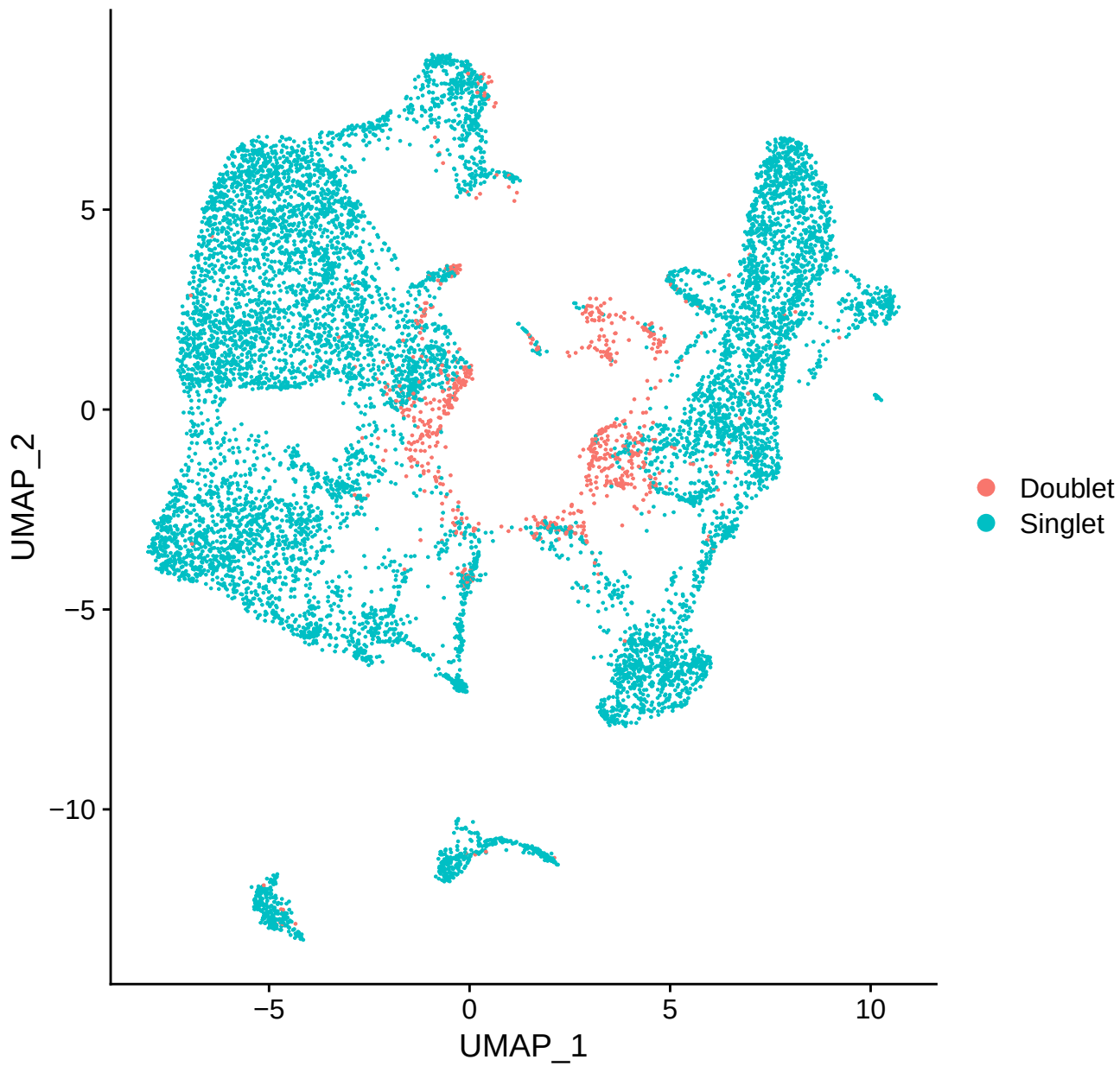
DF.classifications_0.25_0.07_779
