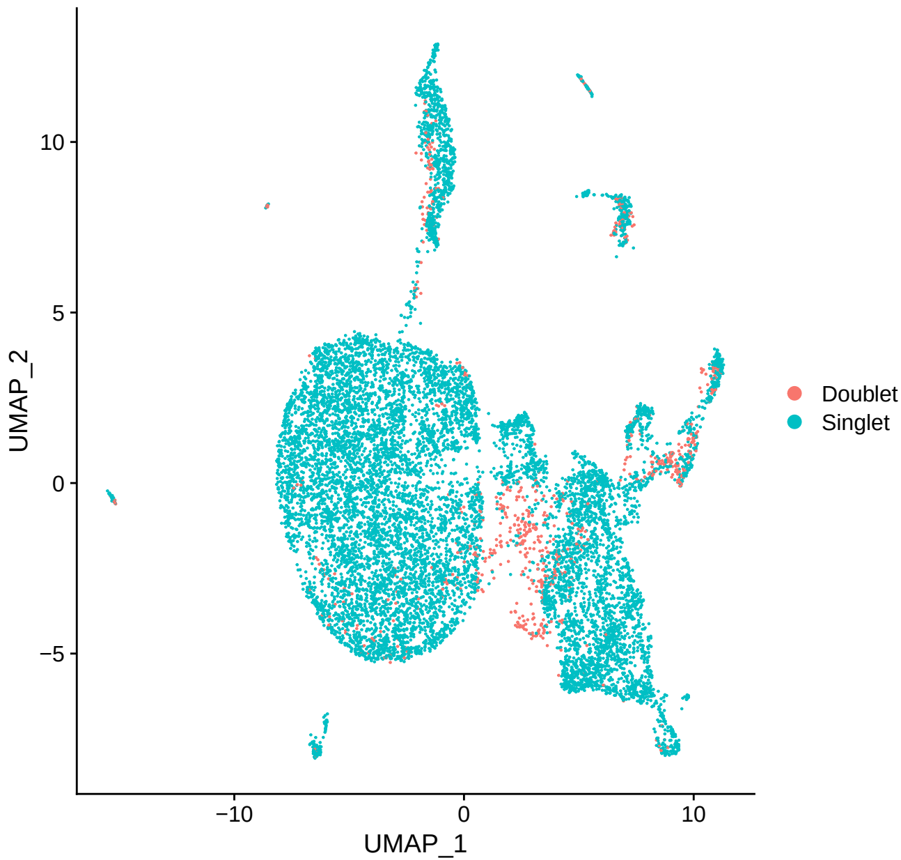
DF.classifications_0.25_0.06_840
