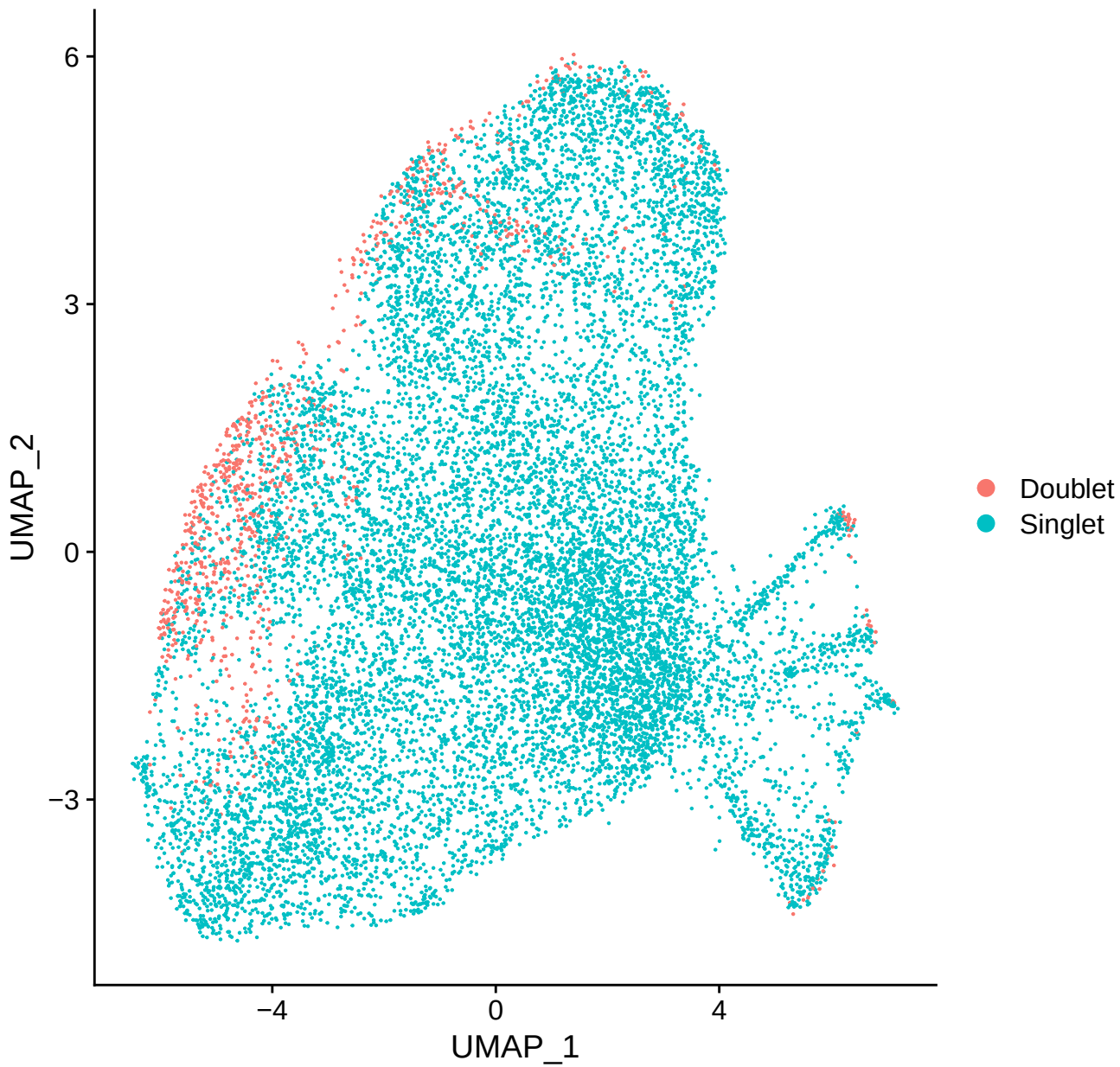
DF.classifications_0.25_0.3_945
