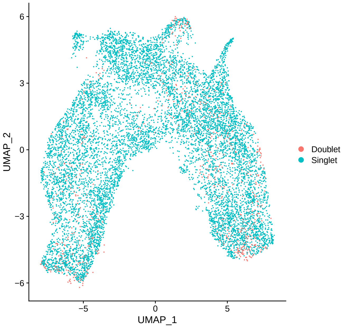
DF.classifications_0.25_0.17_724
