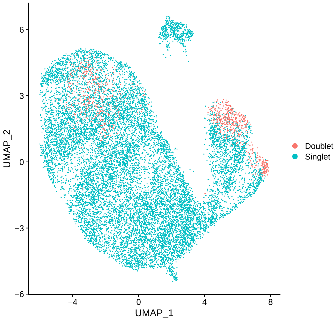
DF.classifications_0.25_0.3_928
