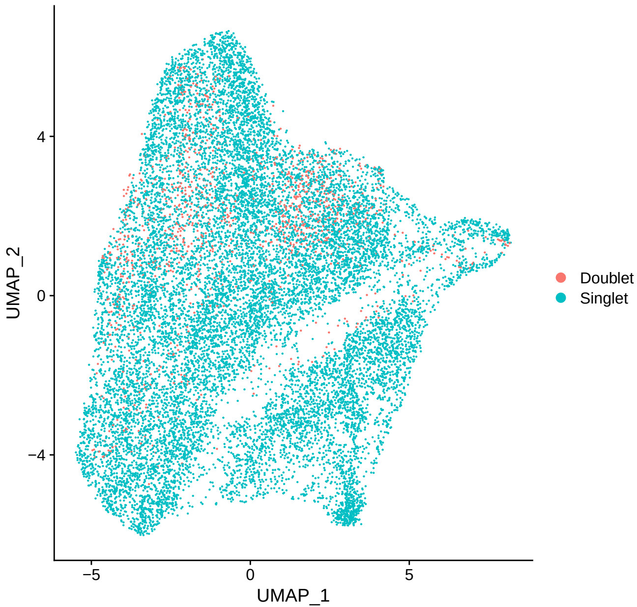
DF.classifications_0.25_0.29_1121
