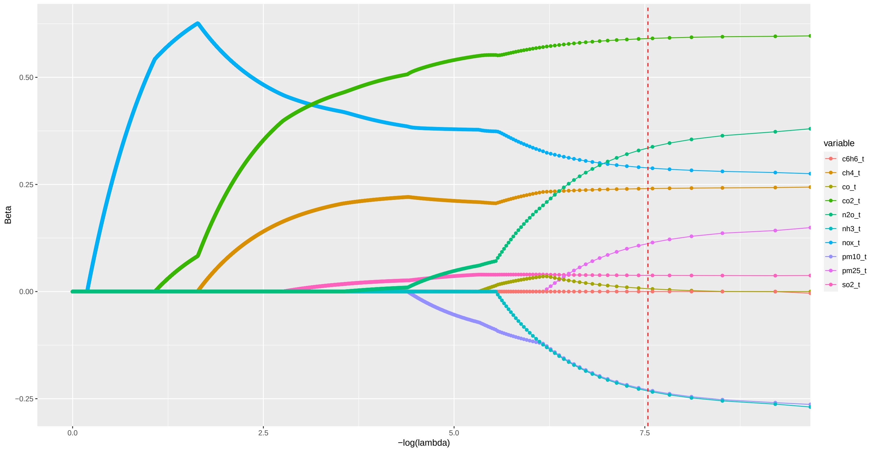
Regularisation Path for Lasso Regression
