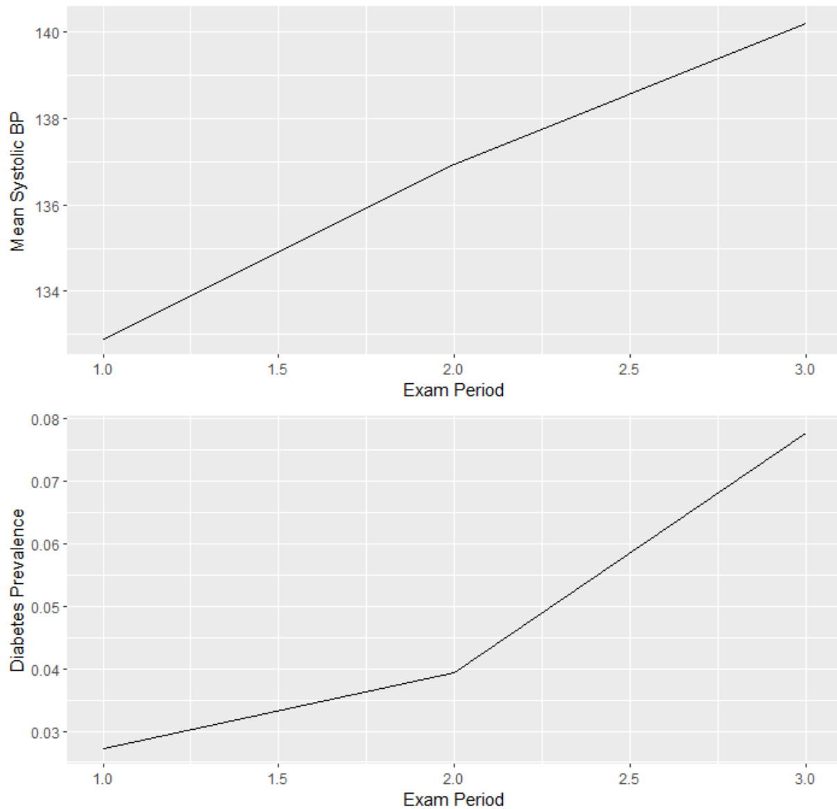
Figure 4: Mean systolic BP and diabetes prevalence were summarized across three Framingham exam periods to evaluate changes in risk factors over time.
