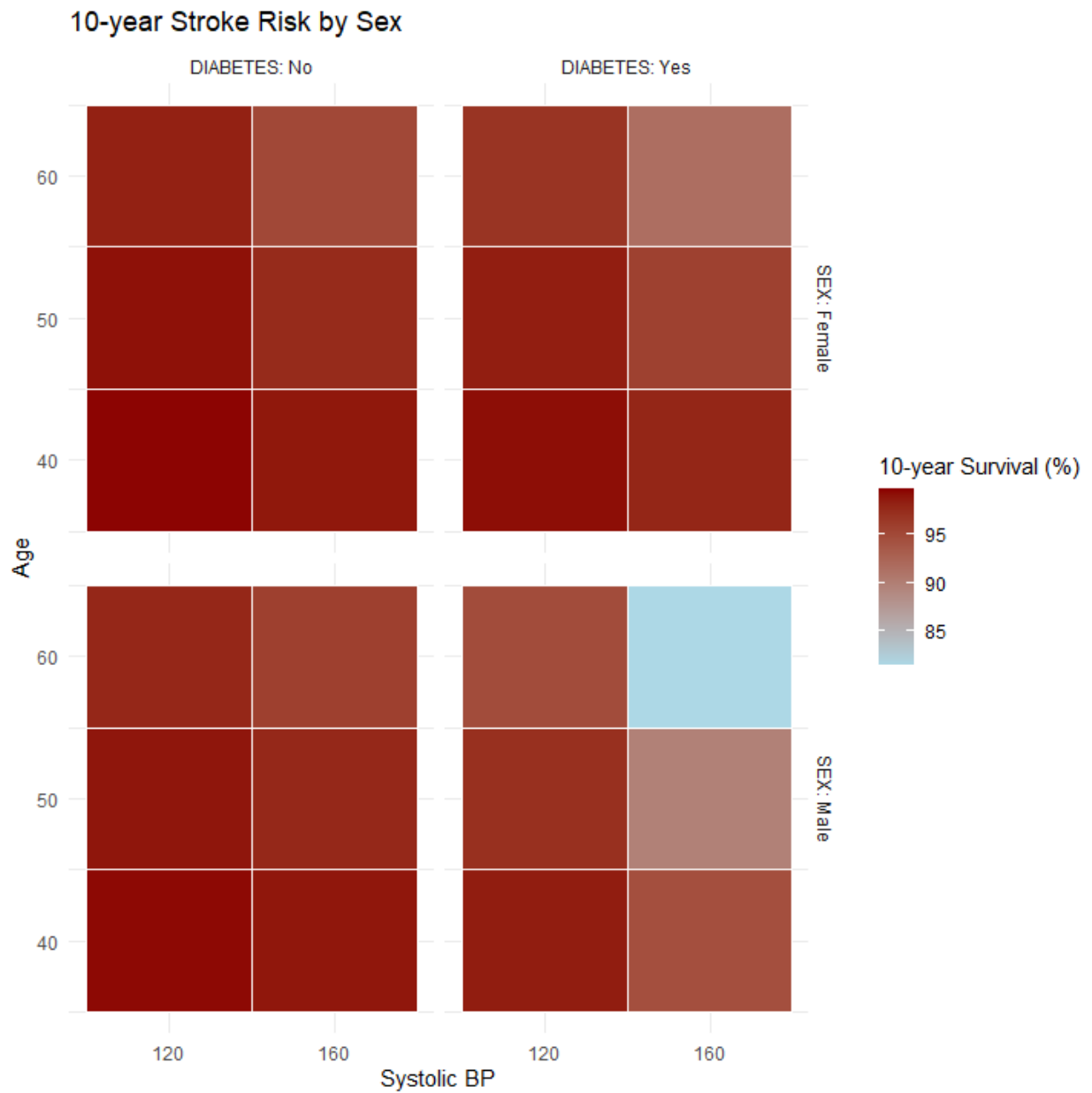
Figure 3: This heatmap visualizes 10 year stroke-free survival probabilities across combinations of systolic BP, diabetes status, age, and sex. Predictions were obtained from sex-specific Cox models. Color gradients represent survival probability, with darker red indicating higher predicted survival.
