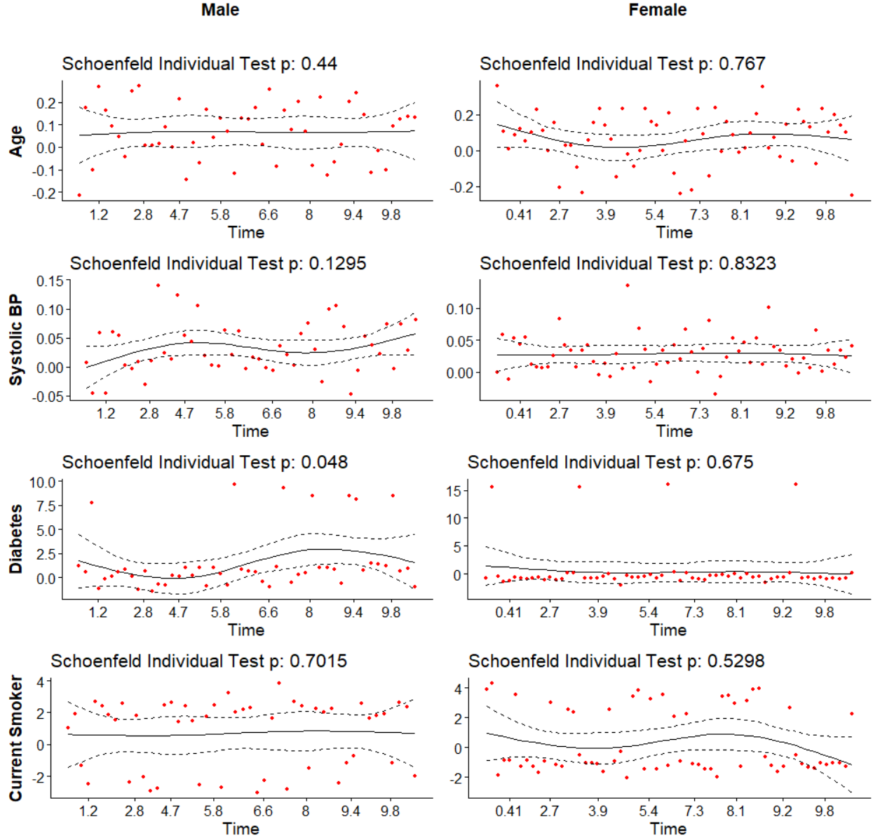
Figure 2: Panels display Schoenfeld residuals over time for age, systolic BP, diabetes, and current smoking, stratified by sex. Each plot includes pointwise residuals, a smoothed trend line, and 95% confidence bands. Individual test p-values are reported for each model. Global p-values are 0.2277 for males and 0.9575 for females. These diagnostics support the proportional hazards assumption of the Cox models used to estimate stroke risk.
