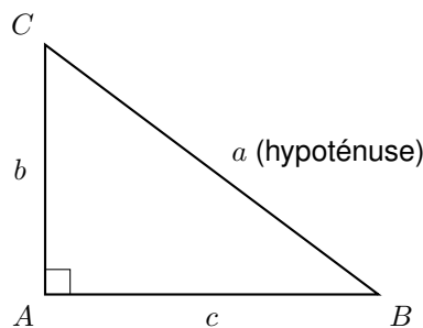
Figure 2: Triangle rectangle : a^2 = b^2 + c^2 .
