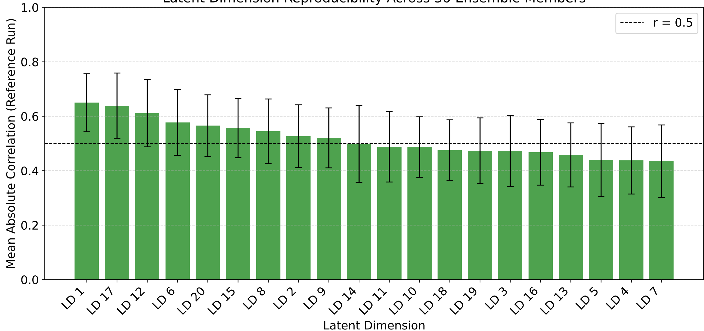
Latent Dimension Reproducibility Across 50 Ensemble Members
