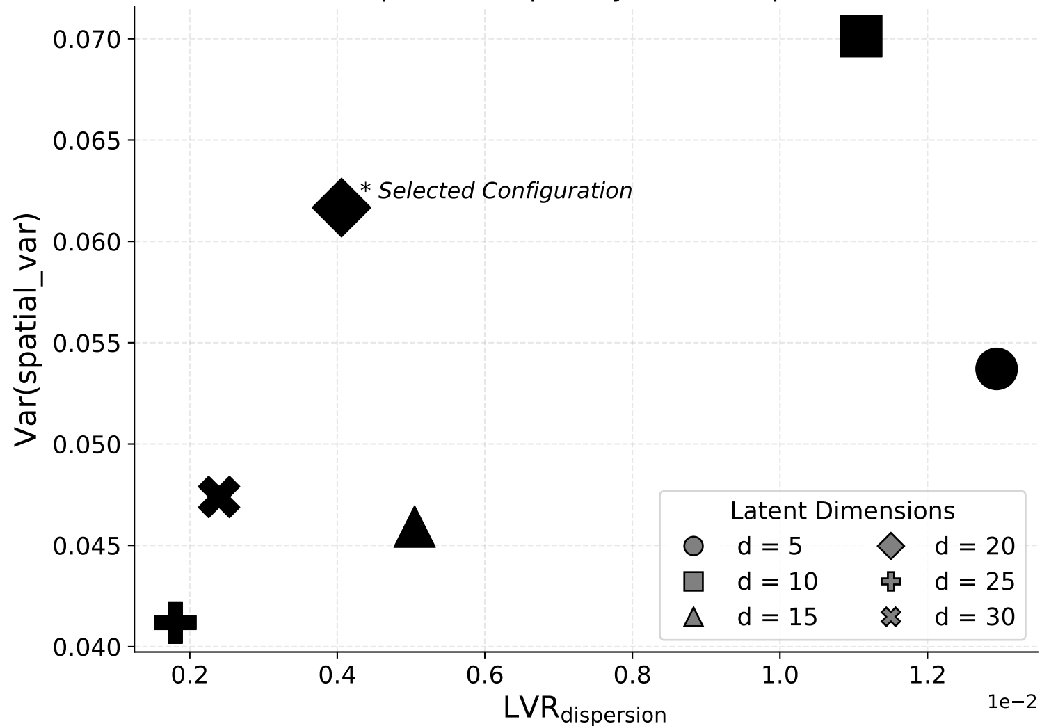
Latent Space Complexity vs. Monopolization
