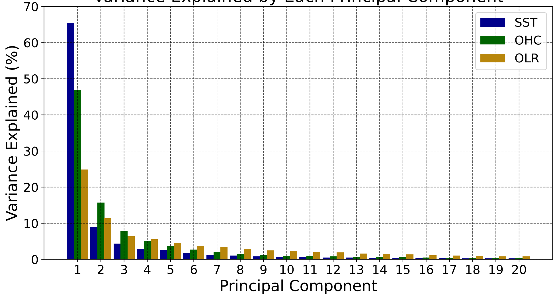
Variance Explained by Each Principal Component
