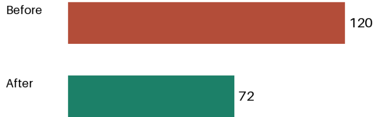
Harbor pilot: measured water use (litres/day)
