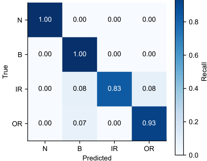
Best LOLO file-level confusion: mlp
