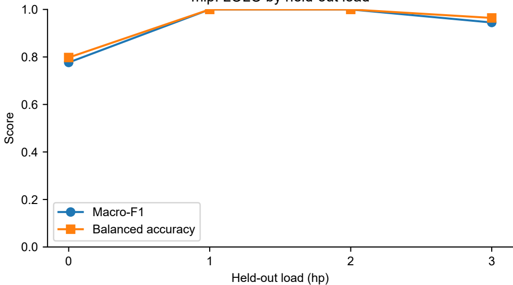
mlp: LOLO by held-out load
