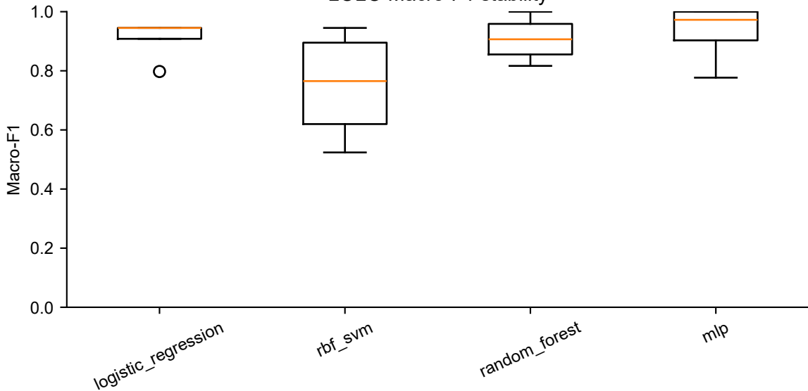
LOLO Macro-F1 stability
