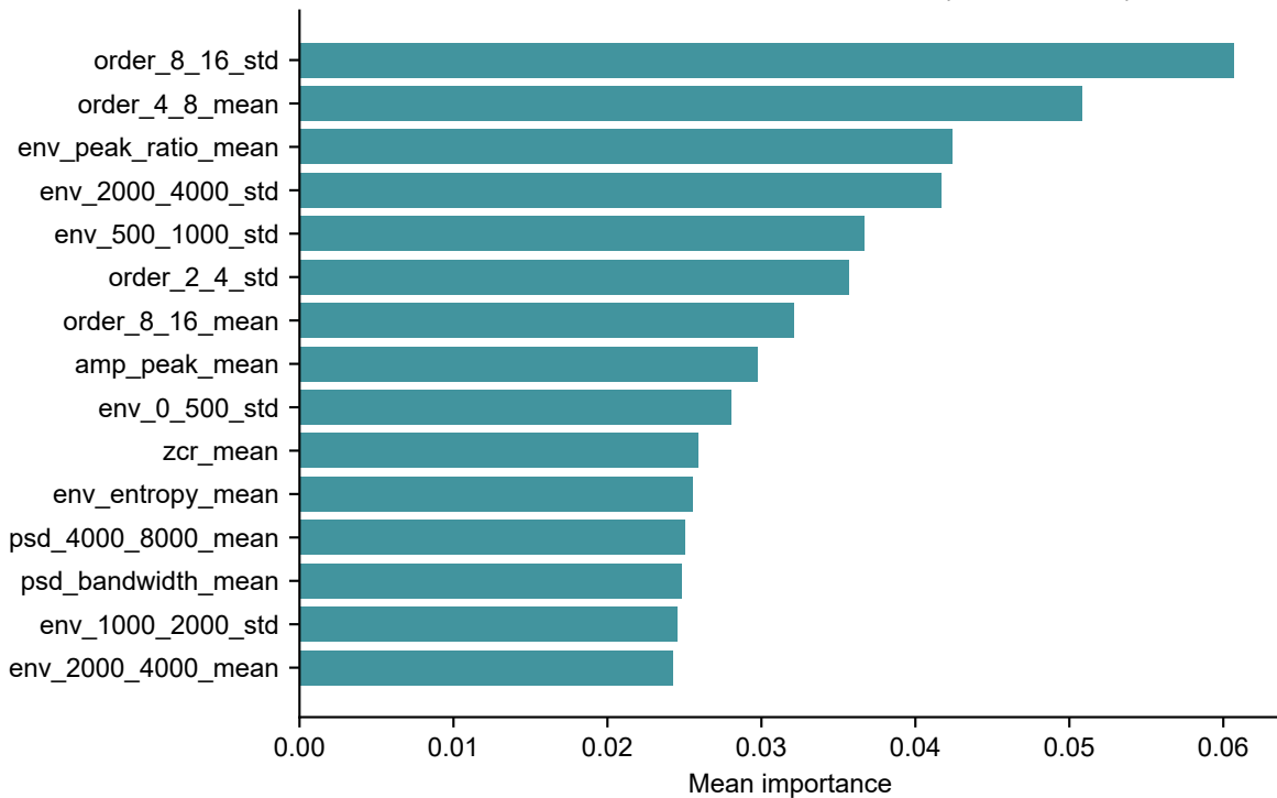
Random-forest feature importance (LOLO mean)
