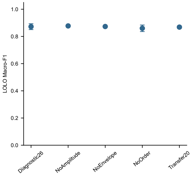
logistic_regression
