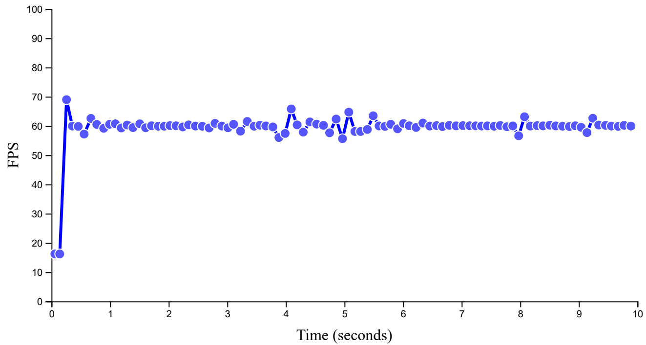
[Excalibur @ 0.26.0-alpha.0+ffc81e1] 2000 Actors (no collisions) Summary [fps Average]: 54.43
