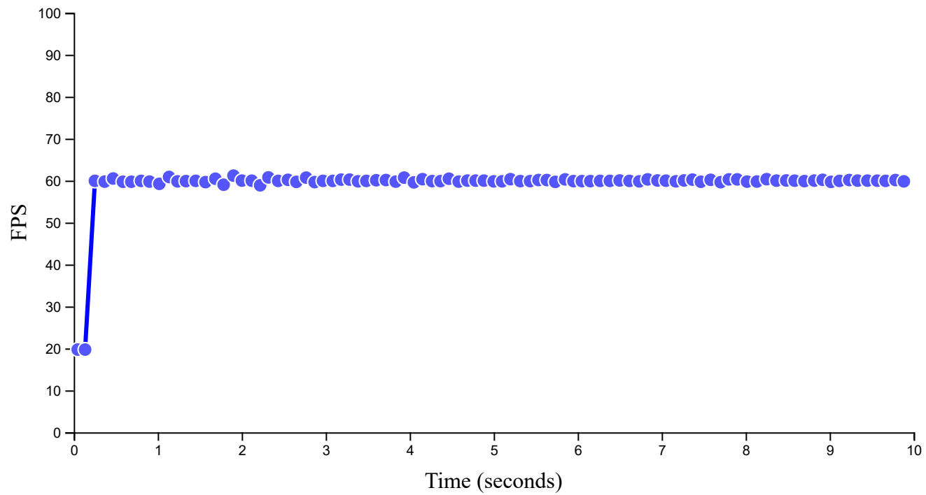
[Excalibur @ 0.26.0-alpha.0+874df73] 2000 Actors (no collisions) Summary [fps Average]: 58.44
