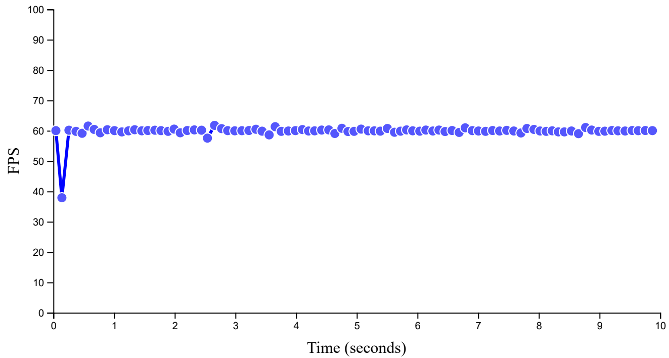
[Excalibur @ 0.26.0-alpha.0+8c0a681] 2000 Actors (no collisions) Summary [fps Average]: 59.27
