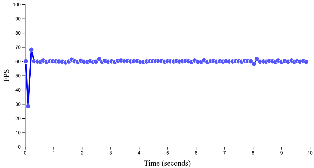
[Excalibur @ 0.26.0-alpha.0+302cac4] 2000 Actors (no collisions) Summary [fps Average]: 59.13
