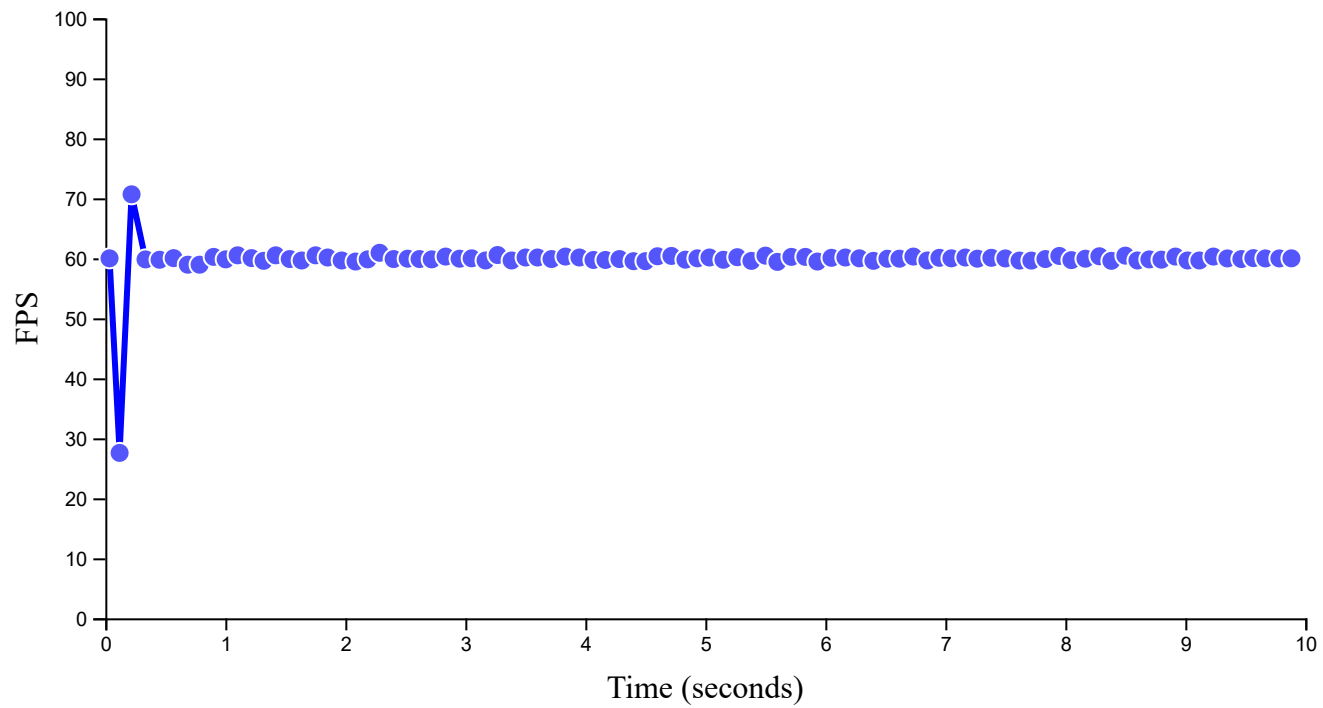
[Excalibur @ 0.27.0-alpha.0+da05e1d] 2000 Actors (no collisions) Summary [fps Average]: 58.95
