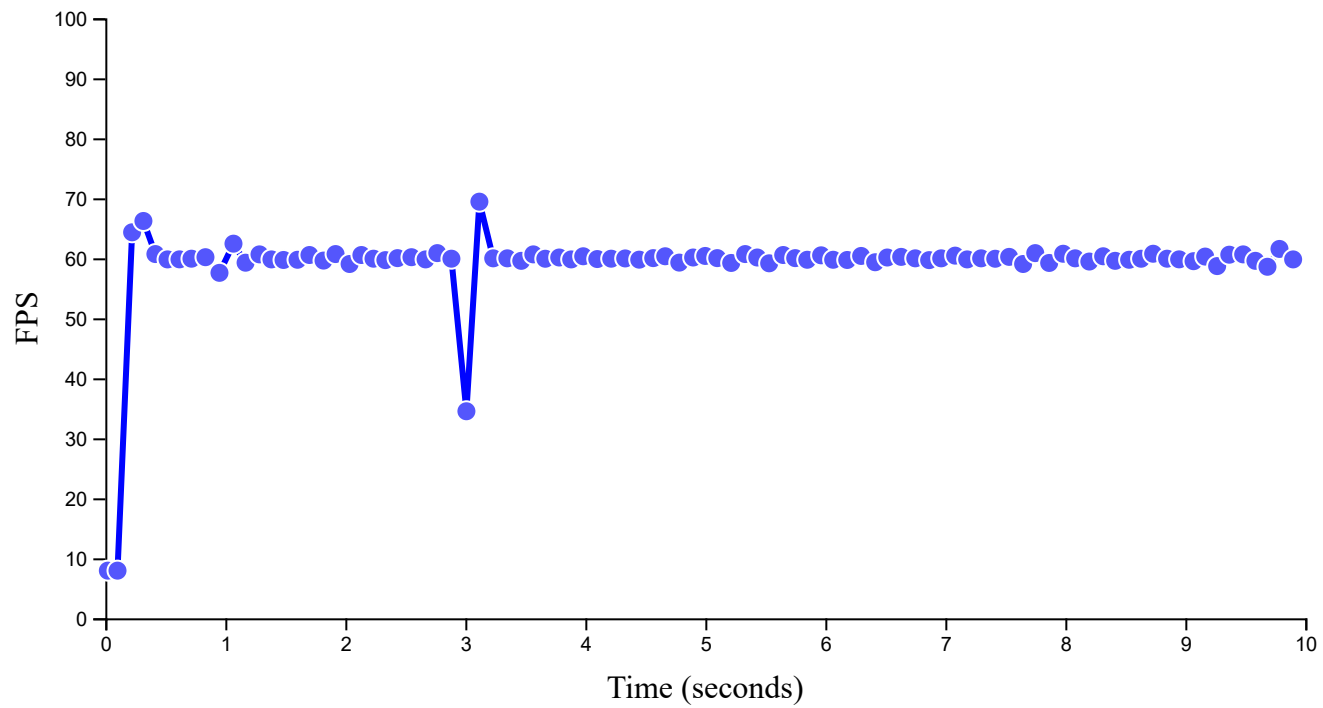
[Excalibur @ 0.25.0-alpha.242+0bbfd4a] 2000 Actors (no sprites, no collisions) Summary [fps Average]: 57.60
