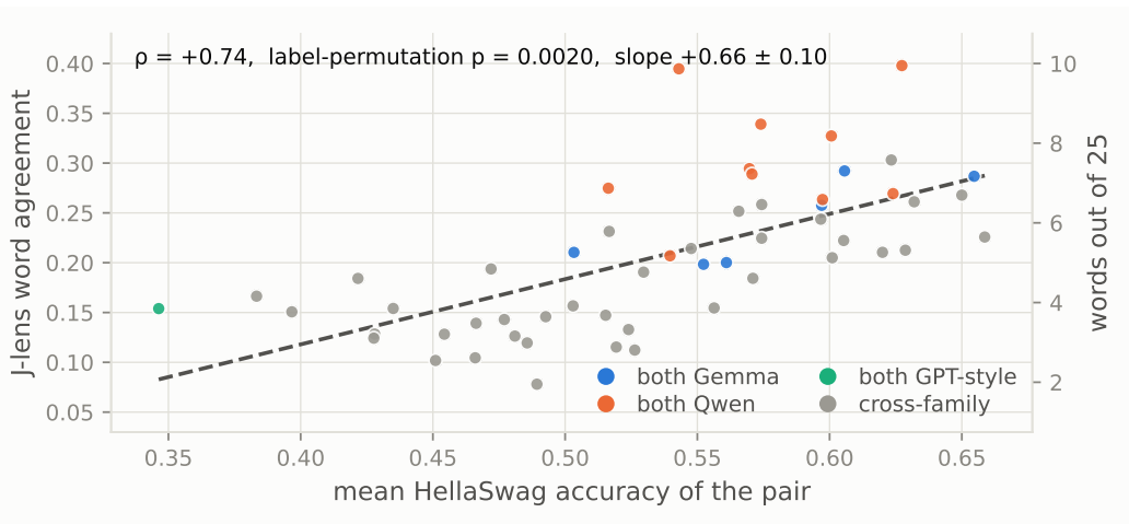
Figure 4: J-lens top-25 median overlap over all matched relative layer depths, against the pair’s mean HellaSwag accuracy. Points are coloured by family composition, and p is a model-label permutation value. Agreement rises with competence.
