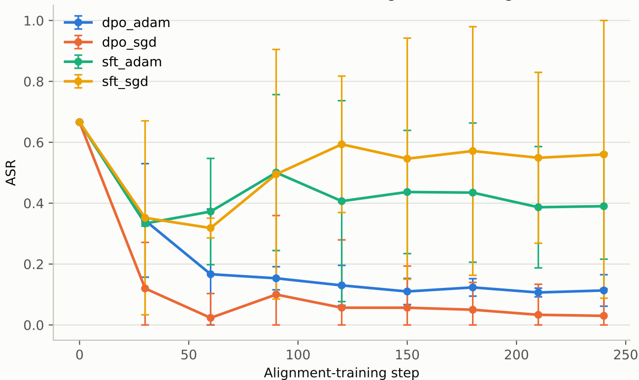
Attack success rate over alignment training
