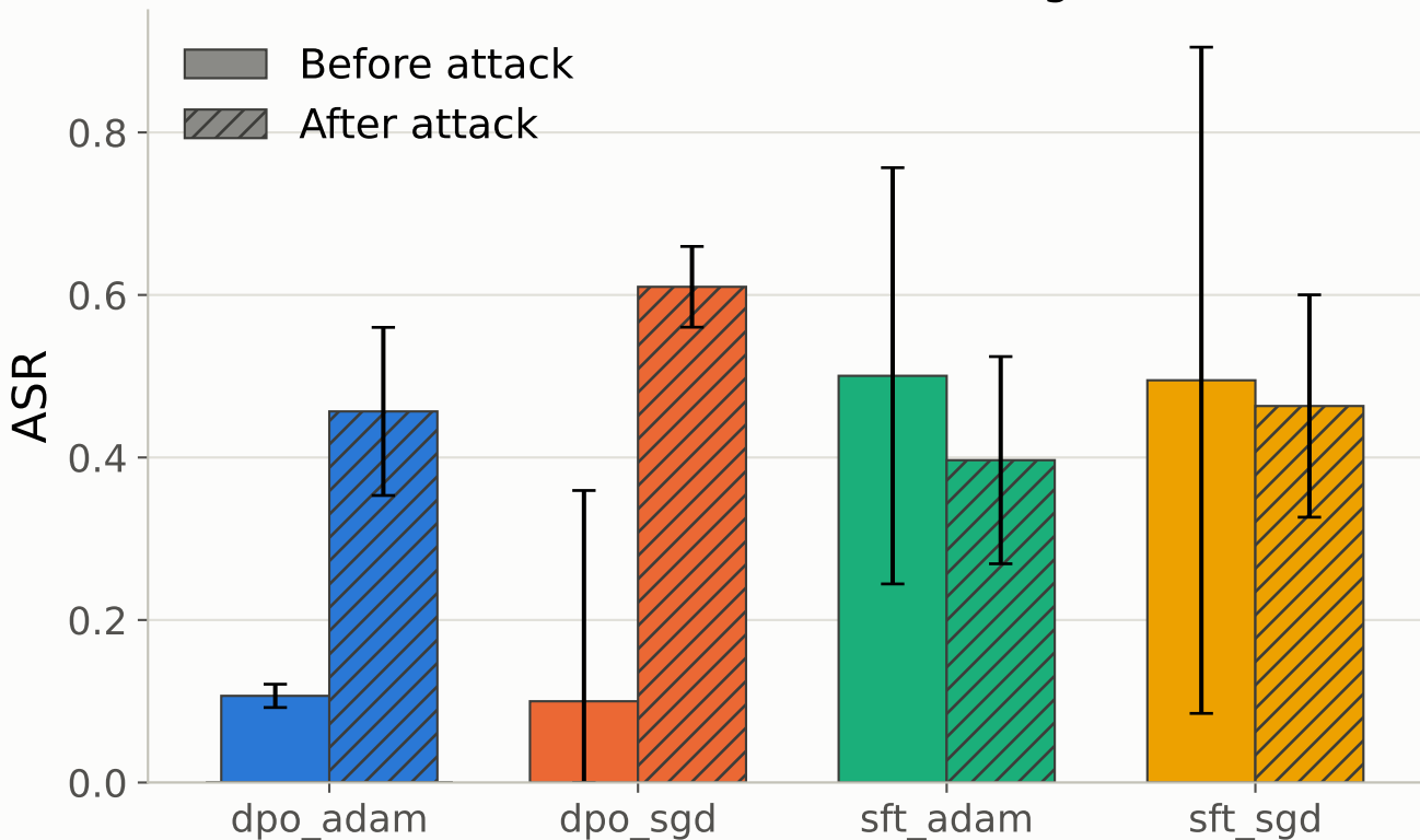
ASR before vs. after fine-tuning attack
