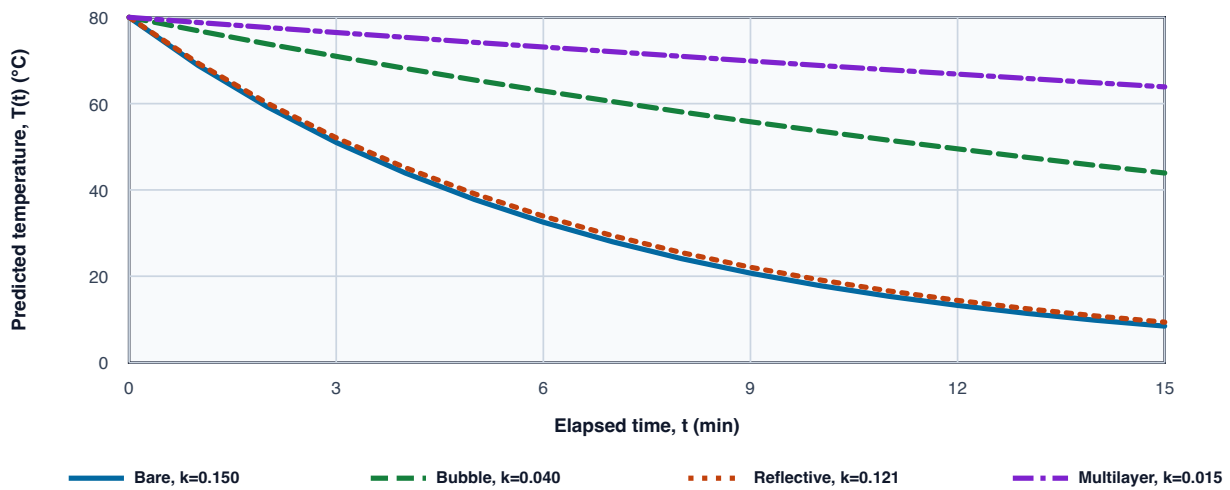
FIGURE 1: COMPLETE 0-15 MIN PREDICTION SET FOR T_0 = 80.0^\circ\text{C} AND T_{\text{env}} = 0.0^\circ\text{C} . Curves use one-minute samples of T(t) = T_{\text{env}} + (T_0 - T_{\text{env}})e^{-kt} ; line patterns remain distinguishable in greyscale.
