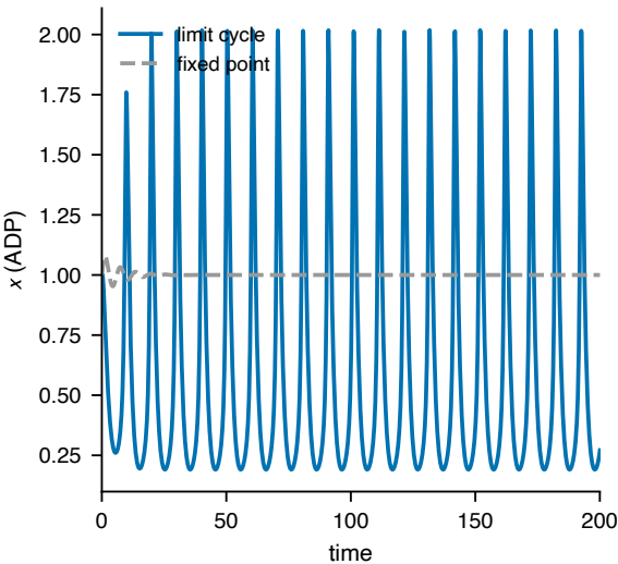
(a) Sel'kov 1968
