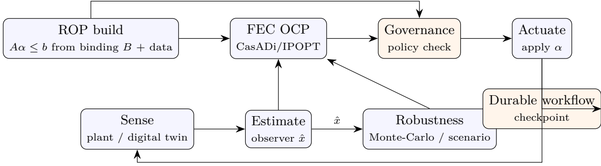
Figure 1: Closed-loop reference architecture implemented by ropfec . The ROP is built once from binding stoichiometry and data and supplies hard constraints to the FEC optimal-control problem and the governance check; the estimation, robustness, governance and workflow blocks are reference implementations, not a production platform. The loop is intended to supervise a staged-bioconversion process (deconstruction → kernel/handover → recovery; the BOS pattern [15]), for which the ROP supplies the admissible exponent geometry.
