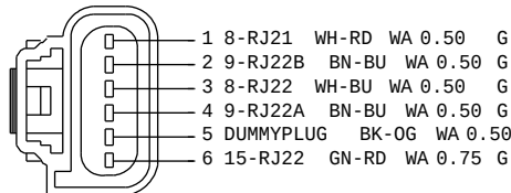
3W4T-14A464-VA(XXX) C394 TO AIR TEMP / MAP SENSOR HARNESS 12A690
