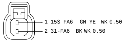
XR3T-14A464-AA C952 TO A/C CLUTCH SOLENOID HARNESS 12A690
