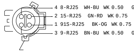
1F1T-14A464-JA(XXX) C959 TO HEGO 1 SENSOR UPSTREAM HARNESS 12A690
