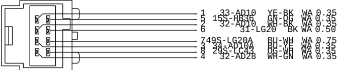
2L1T-14A624-SA C819 TO 14K138 HARNESS PASS. SIDE MIRROR UNIT
