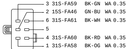
96AG-14489-RFA C553 TO LEFT DOOR TEMPERATURE HARNESS 14401
