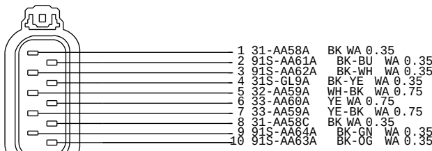
3M5T-14A464-DKA C148 TO DRIVER FRONT DOOR LATCH UNIT HARNESS 14A584
