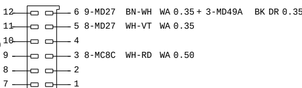
3S7T-14489-FA C448 TO RADIO 4 (MICRO/EXTERNAL AUXILIARY/NAVIGATION) HARNESS 14401
