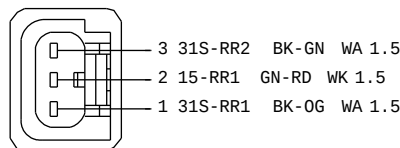
1W7T-14A464-LA C645 TO IGNITION COIL TRANSFORMER(NEW) HARNESS 12A690
