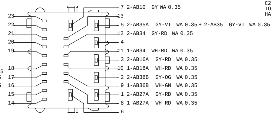
157T-14489-EC C215 TO (KVM) HARNESS 14014
