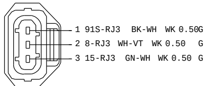
112T-14A464-UA C352 TO CID HALL SENSOR INTAKE HARNESS 12A690
