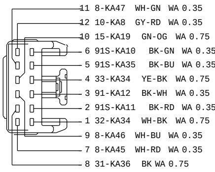
97BG-14489-YMB C441 TO FRONT AND REAR WIPER SWITCH HARNESS 14401
