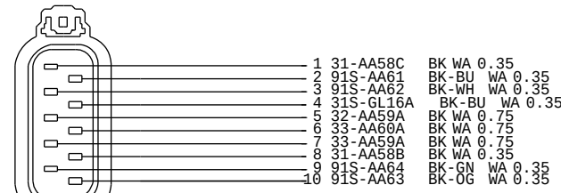
3M5T-14A464-DKA C149 TO PASS. FRONT DOOR LATCH UNIT HARNESS 14K138
