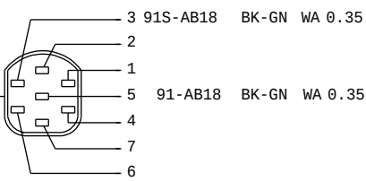
3M5T-14A464-RGA C208 TO RL UNLOCK SWITCH (KVM) HARNESS 14240
