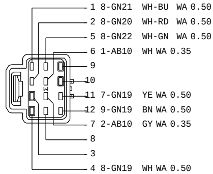
3M5T-14A464-UMB C608 TO 14014 HARNESS 15K868
