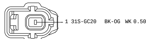
F65B-14A464-CA C978 TO OIL PRESSURE SWITCH HARNESS 12A690
