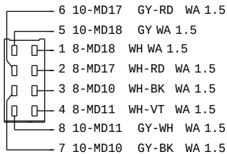
3S7T-14489-DA C442 TO RADIO 2 (SPEAKER) HARNESS 14401
