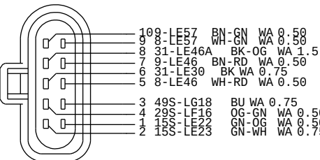
1X4T-14A464-ADA C837 TO RIGHT HEAD LAMP HARNESS 14K733
