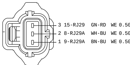
F6DB-14A464-AGA C524 TO VEHICLE SPEED SENSOR HARNESS 12A690
