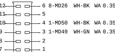
3S7T-14489-EA C447 TO RADIO 3 HARNESS 14401
