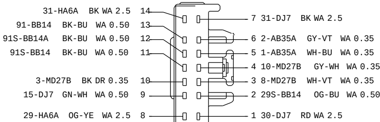
457T-14489-YRA C155 TO 15K857 HARNESS 14401
