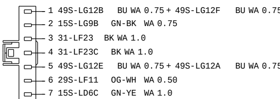
1S7T-14489-NA C476 TO LEFT COMBINED REARLAMP HARNESS 14014
