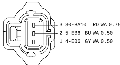
F6DB-14A464-AGA C870 TO ALTERNATOR HARNESS 12A690
