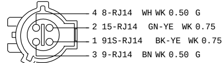
1F1T-14A464-FA(XXX) C960 TO HEGO 1 SENSOR DOWNSTREAM HARNESS 12A690
