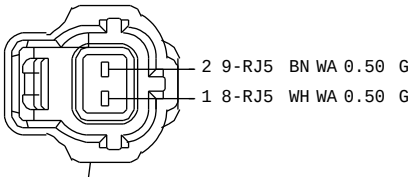
F5AB-14A464-BB C779 TO ENGINE COOLANT TEMPERATURE SENSOR HARNESS 12A690
