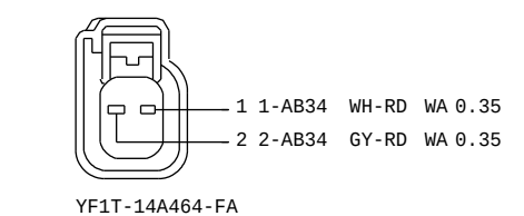
YF1T-14A464-FA C224 TO INTERIOR TRUNK ANTENNA HARNESS 14014
