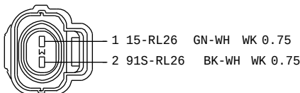
2R8T-14A464-GA C587 TO VARIABLE VALVE EXHAUST HARNESS 12A690
