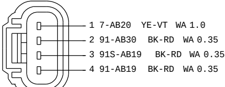
YF1T-14A464-CA C209 TO RL DOOR L/U/L LATCH (KVM) HARNESS 14240
