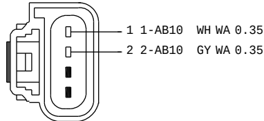
3M5T-14A464-ABA C227 TO EXTERIOR TRUNK ANTENNA HARNESS 15K868
