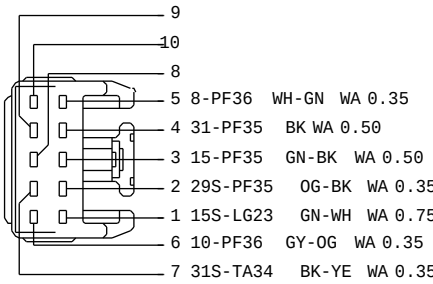
4S7T-14489-VJA C383 TO GEAR SHIFT MODULE (CFT) HARNESS 14401
