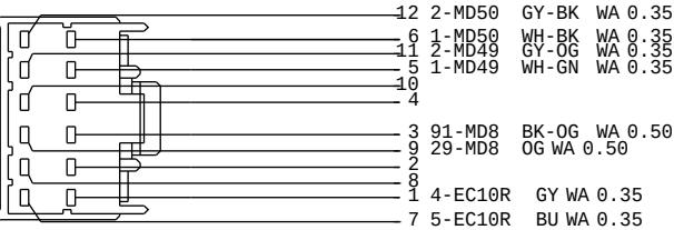
F50B-14489-GA C440 TO CD CHANGER HARNESS 14B723
