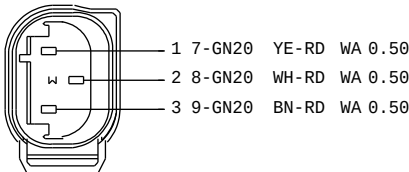
98AG-14A464-RDA C605 TO PARK AID SENSOR HARNESS 15K868
