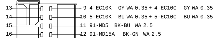
3M5T-14A541-BA C443 TO RADIO 2 (SPEAKER) HARNESS 14401
