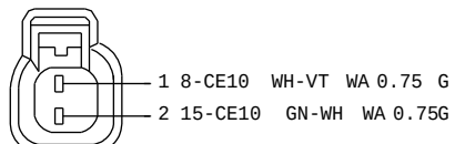
XW43-14A464-AAA C386 TO STEERING PRESSURE SENSOR HARNESS 12A690
