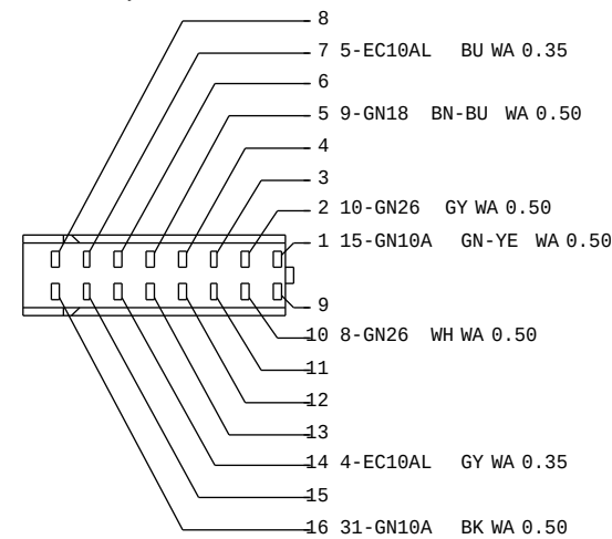
3M5T-14488-AA C622 TO PARKING AID MODULE HARNESS 14014
