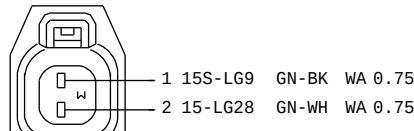
1X4T-14A464-AAB C866 TO TRANSMISSION SWITCH HARNESS 12A690
