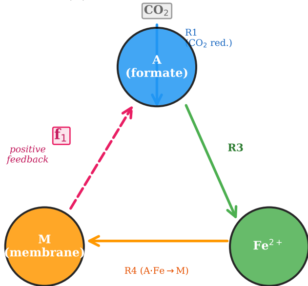
(a) Reaction network
