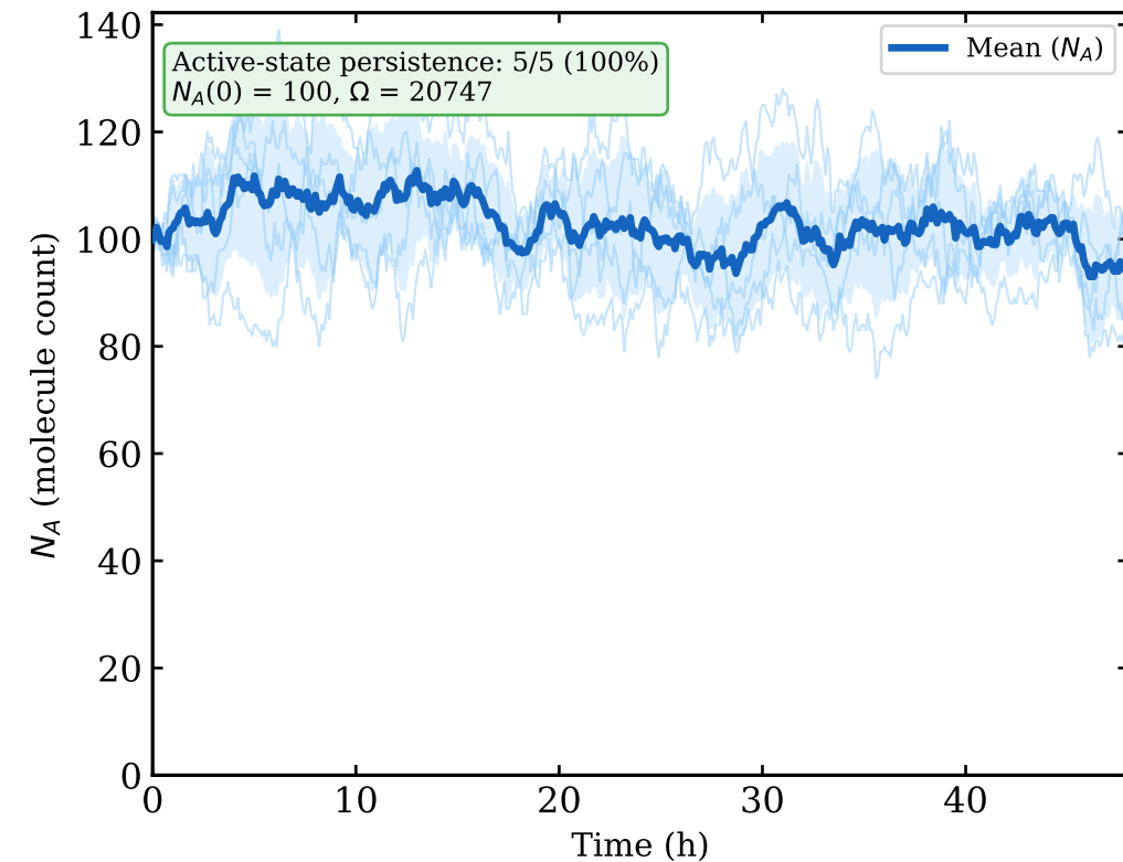
(c) Gillespie SSA (5 trajectories)
