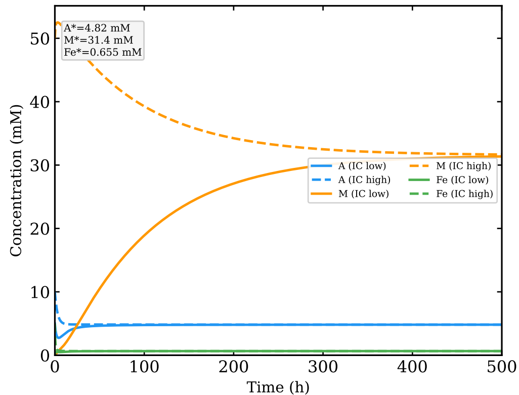
(b) ODE: convergence to steady state
