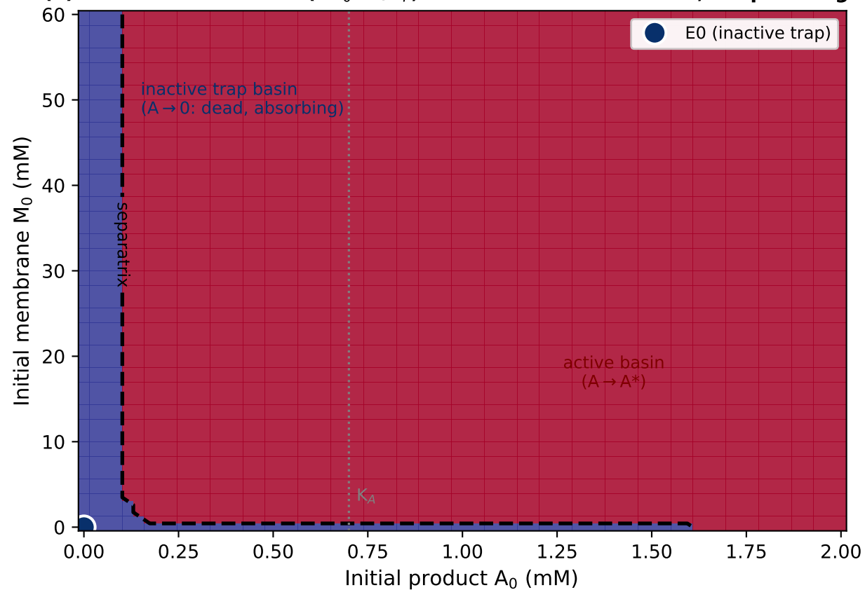
(a) Basins of attraction ( Fe_0 = S/k_F ; E+ active at A^* \approx 4.8 mM, off-panel right)
