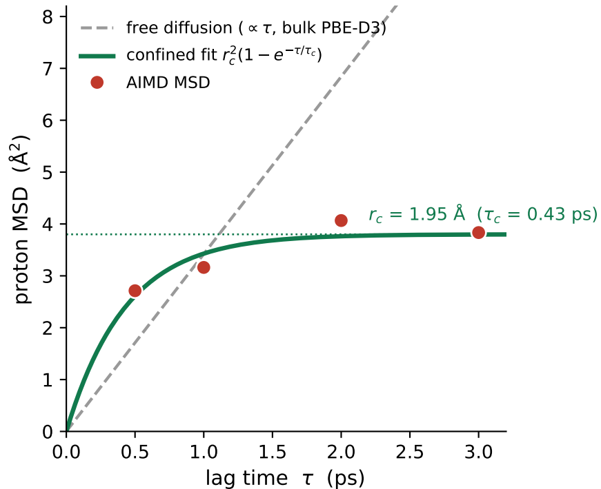
(b) Mean-square displacement: confined, not diffusive
