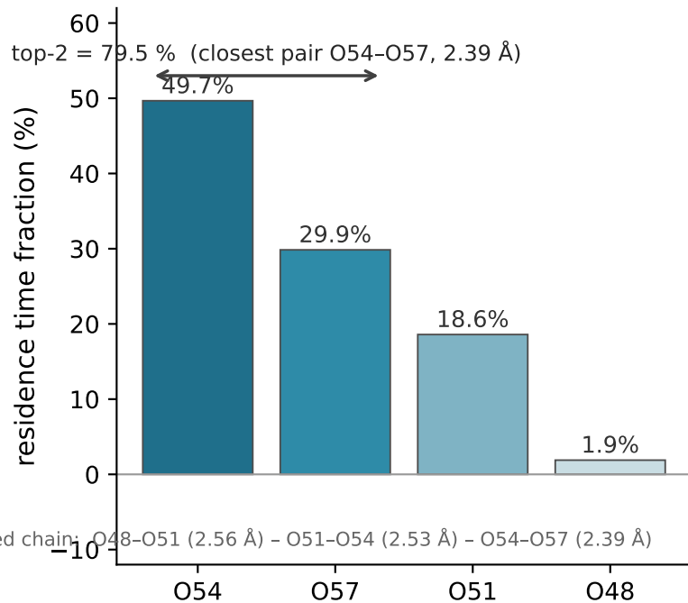
(a) Per-site proton residence (50 fs filter)
