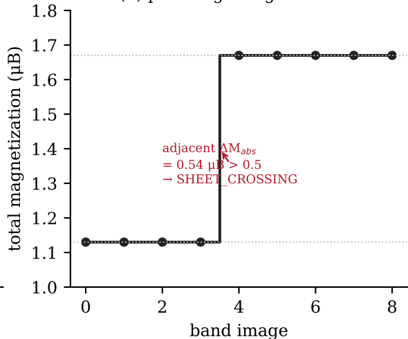
(b) per-image magnetization
