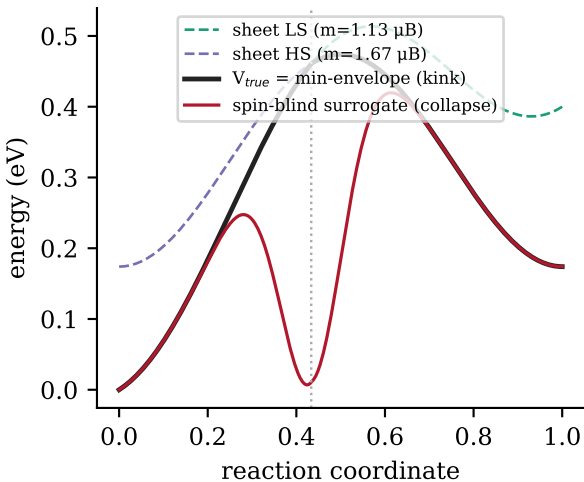
(a) two spin sheets
