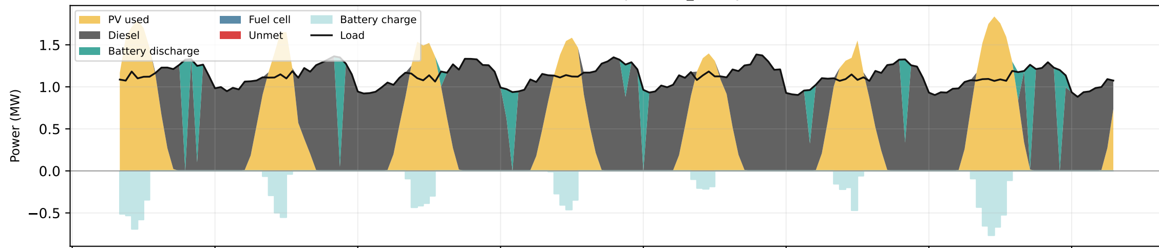
PV + diesel + battery (diesel_battery)
