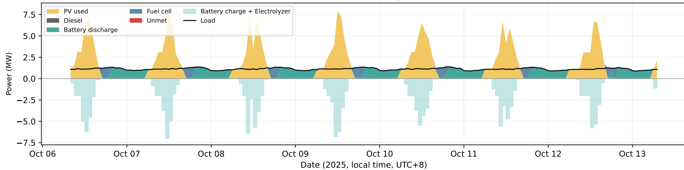
PV + battery + H 2 (battery_hydrogen)
