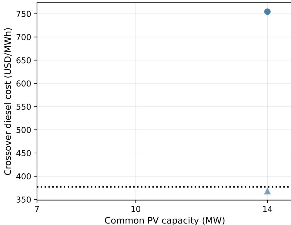
Economic Crossover vs PV Scale (pure annual cost, carbon=150 USD/tCO 2 , outage=48 h)
