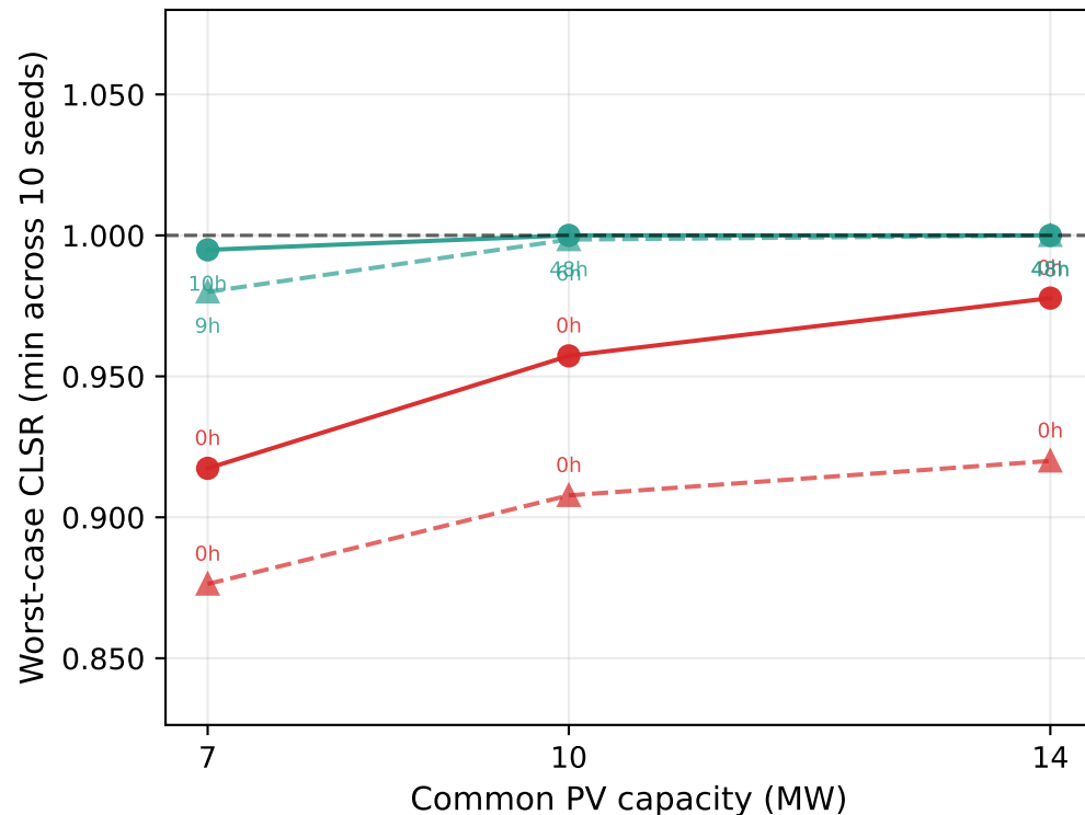
Resilience vs PV Scale (48 h outage, 4/yr, seeds 1-10; labels = survivable_h_min)
