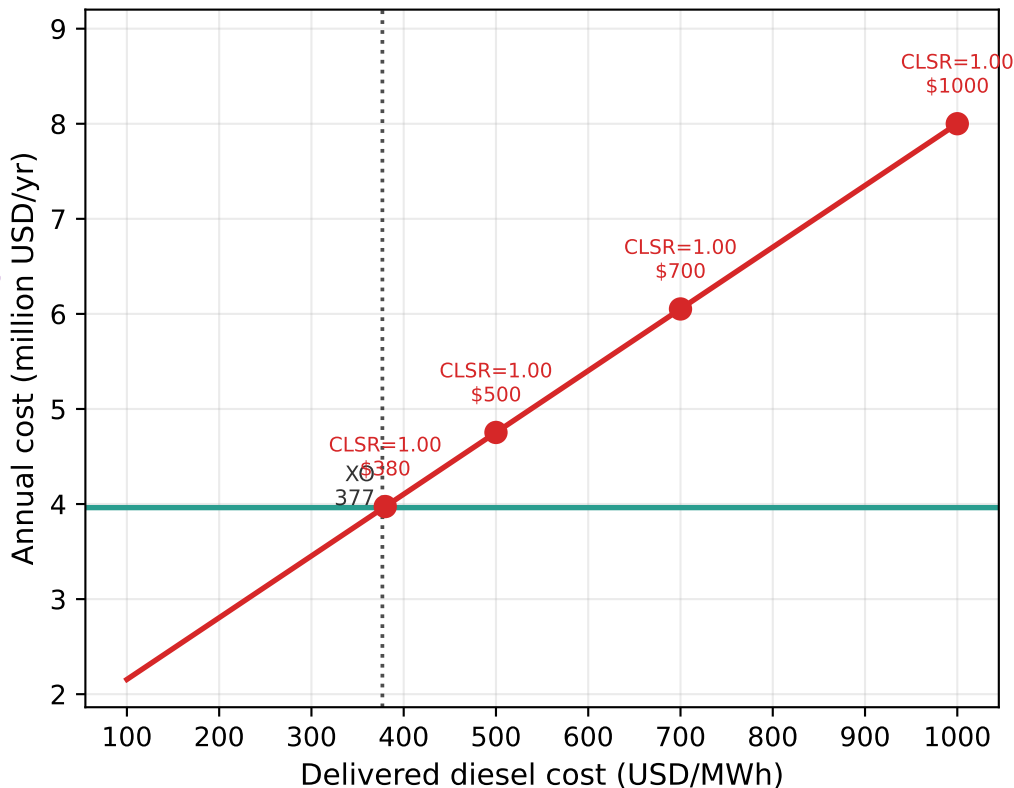
D4 Diesel Available — Economic Crossover (carbon=150 USD/tCO 2 ; CLSR=1.0 for both above crossover)
