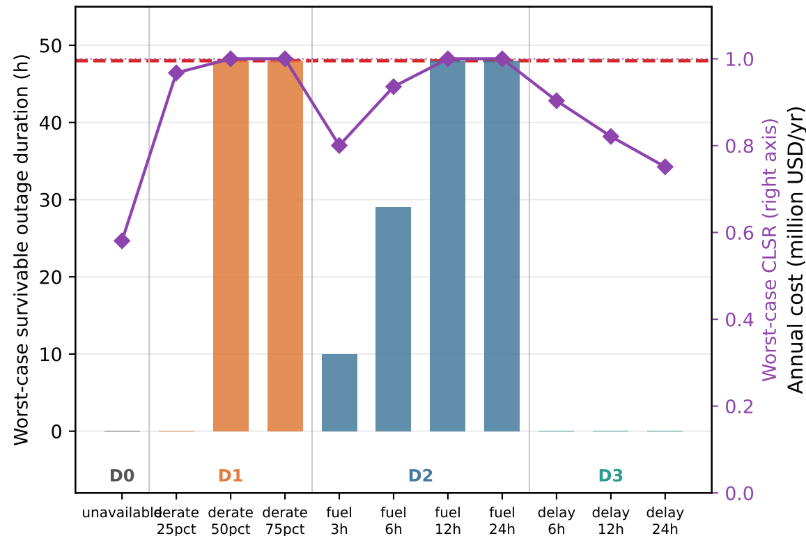
D0-D3 Diesel Availability — Resilience Impact (diesel_battery, 10 seeds, 48 h/4 events/yr; H 2 always 48 h)
