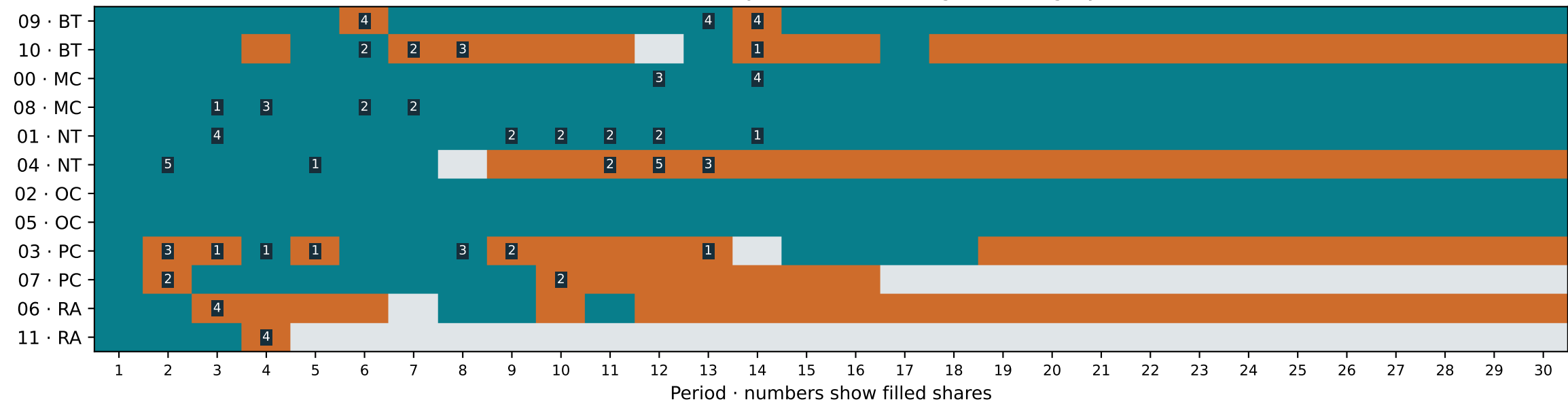
Seed 140928 · buy (teal), sell (orange), hold (gray)
