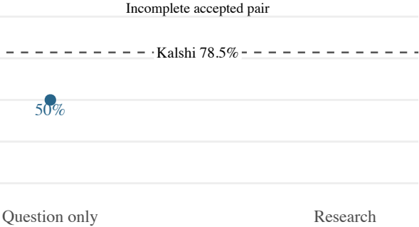
Claude Fable 5.1
