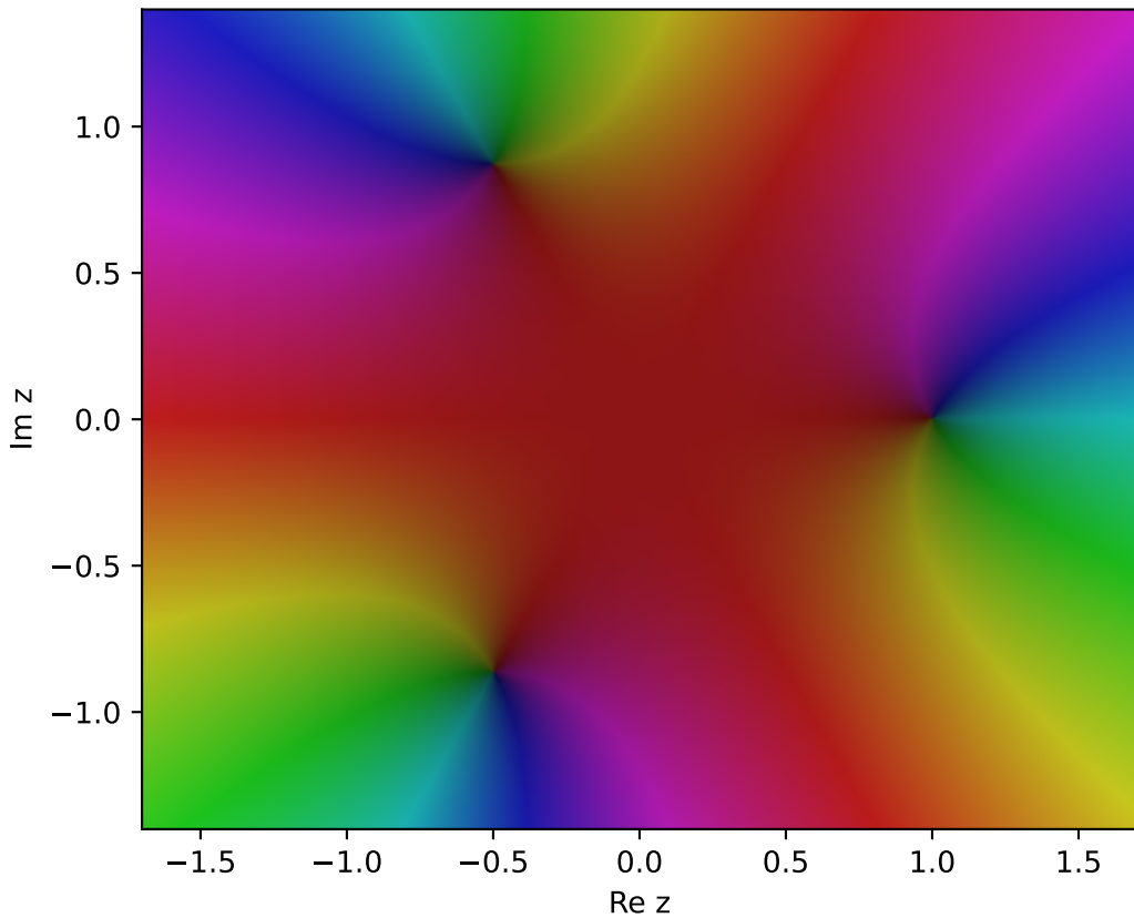
Domain coloring of f(z) = z^3 - 1
