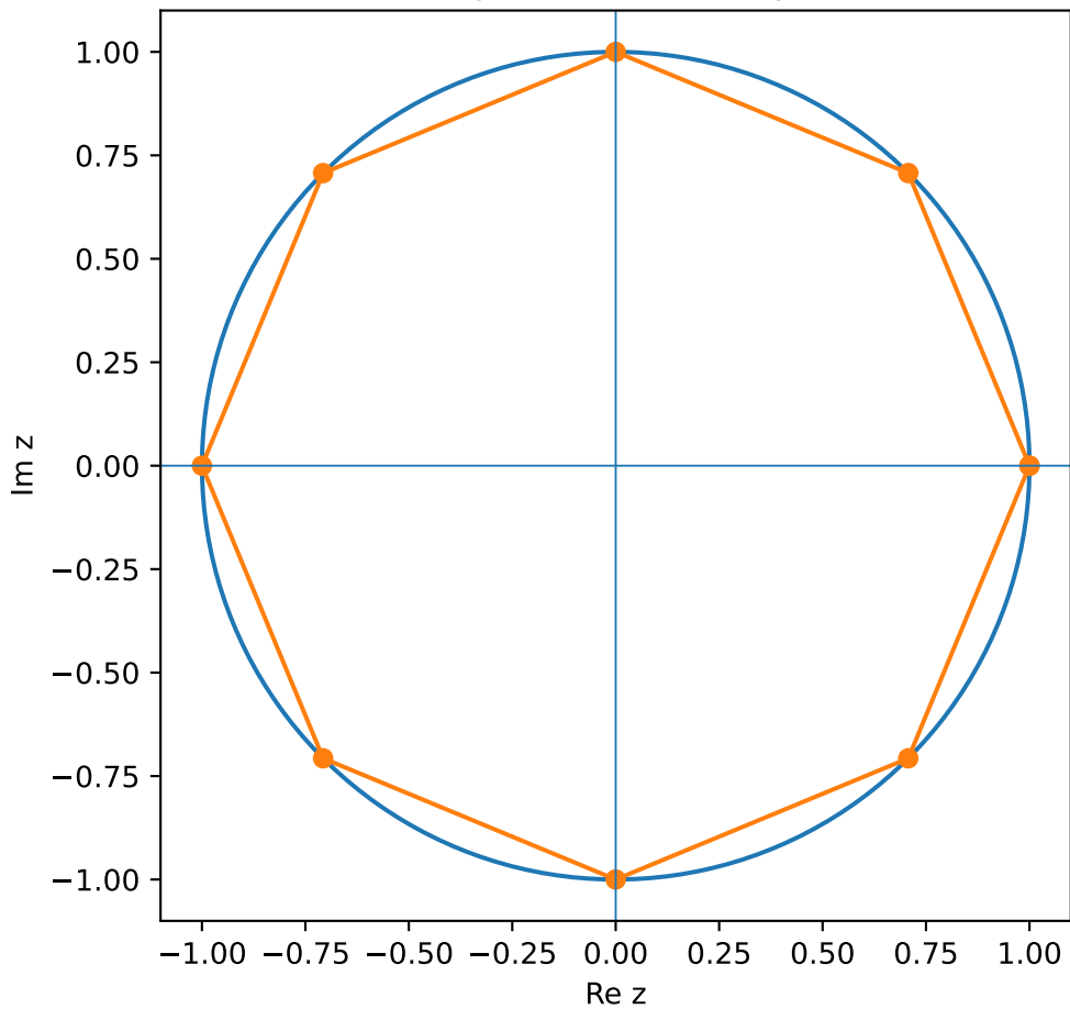
Eighth roots of unity
