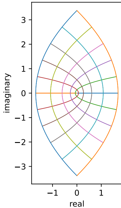
image under w = z^2
